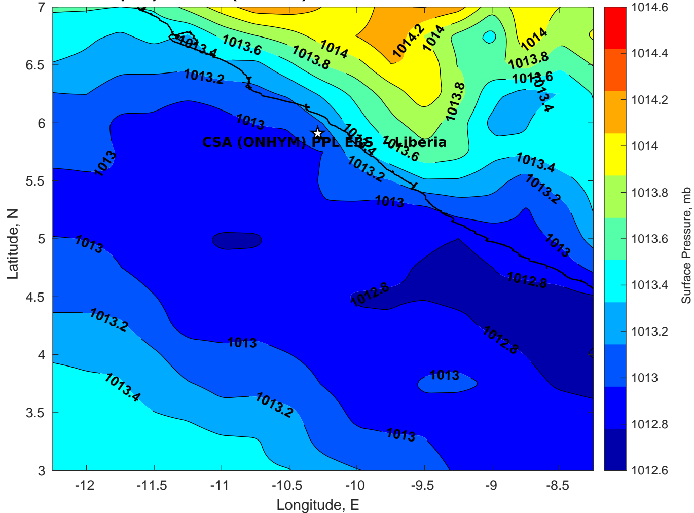
Surface Pressure (mb) for CSA (ONHYM) PPL EBS - Liberia at 24-Mar-2025 00:00:00
