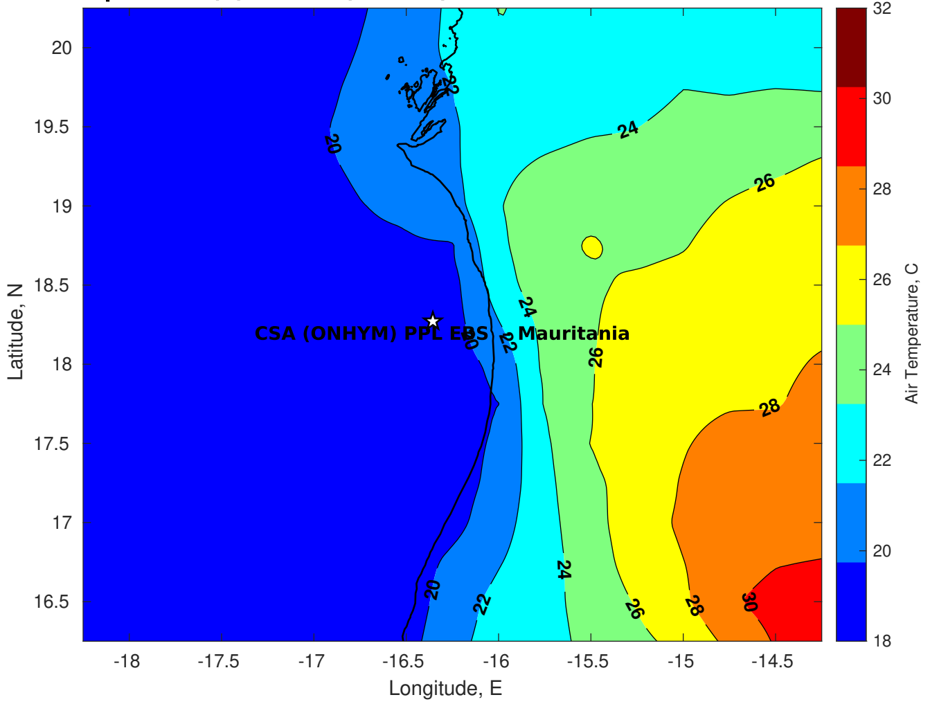
Air Temperature (C) for CSA (ONHYM) PPL EBS - Mauritania at 23-Mar-2025
