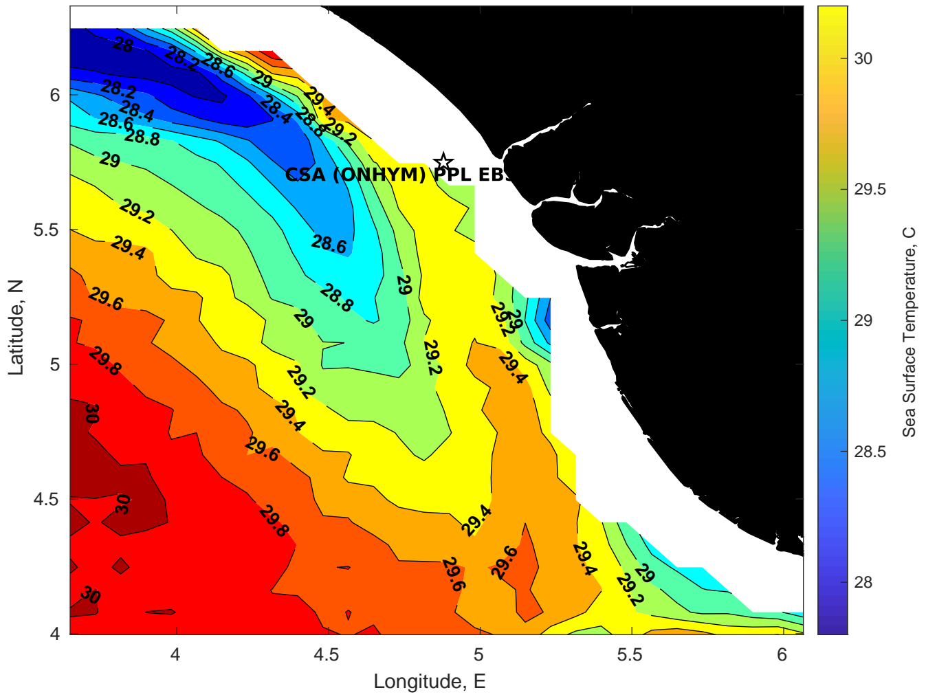
SST for CSA (ONHYM) PPL EBS - Nigeria at 22-Mar-2025 00:00:00
