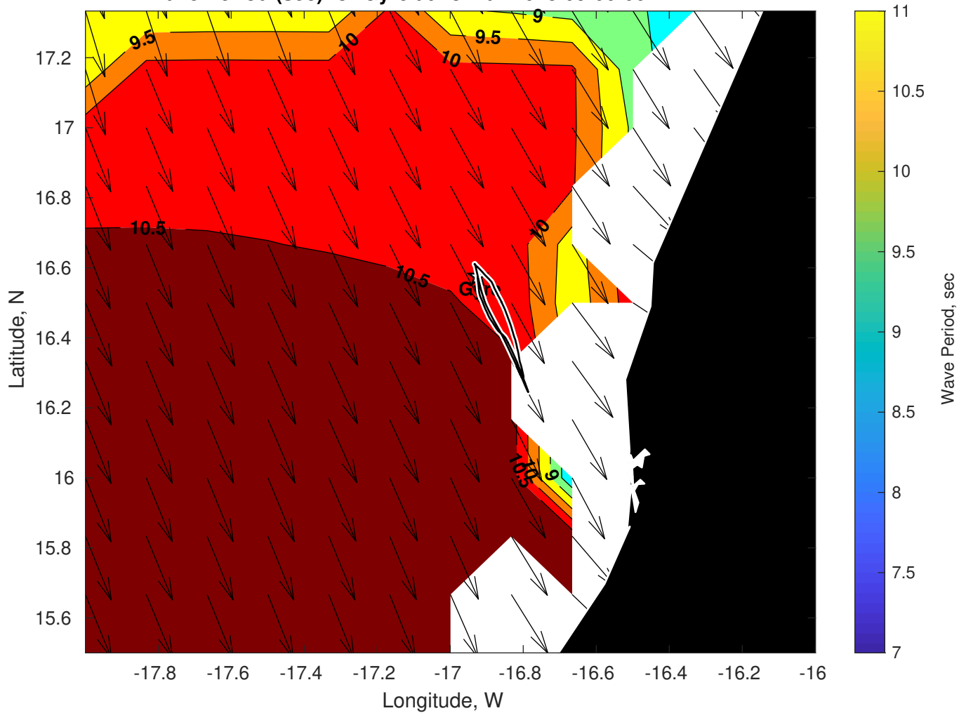
Wave Period (sec) for Gyre at 23-Mar-2025 09:00:00
