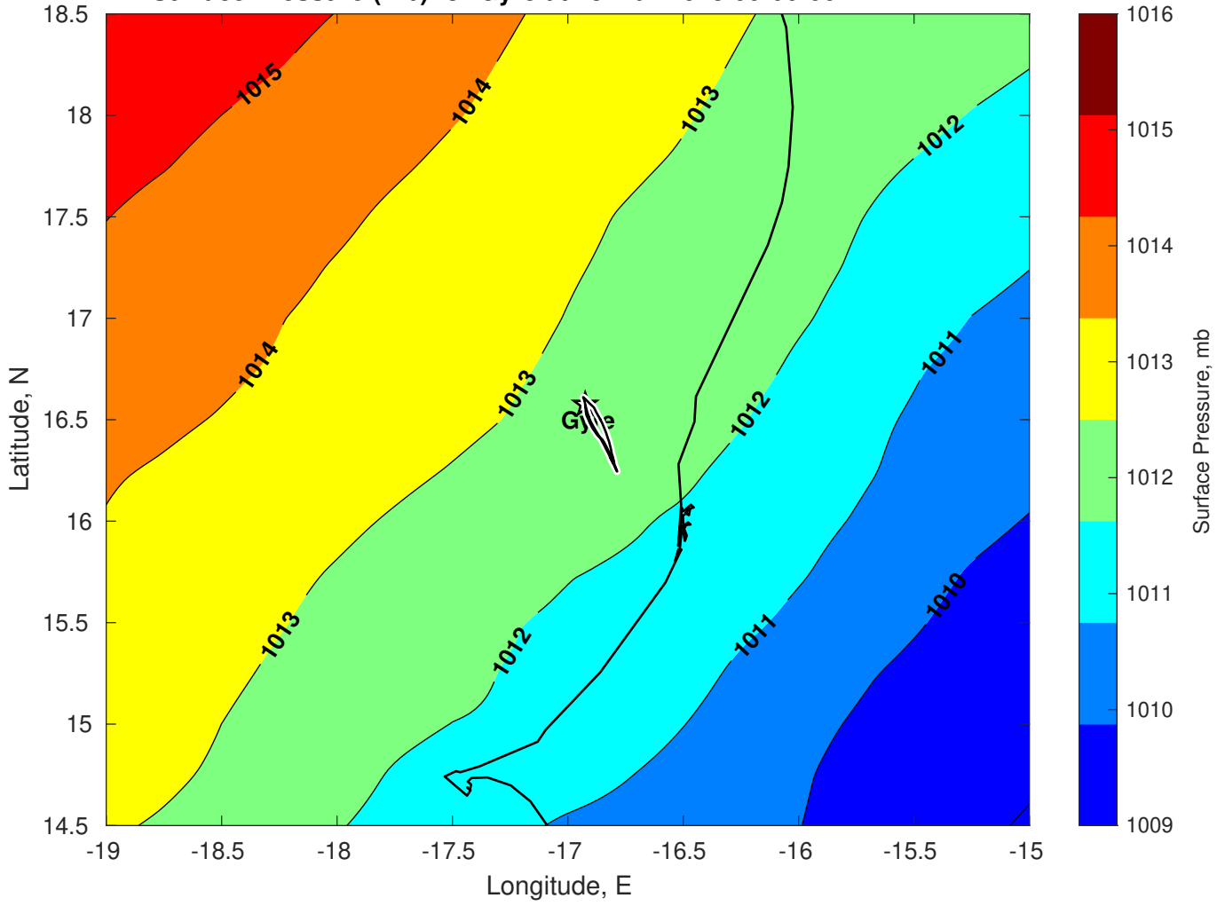
Surface Pressure (mb) for Gyre at 23-Mar-2025 00:00:00
