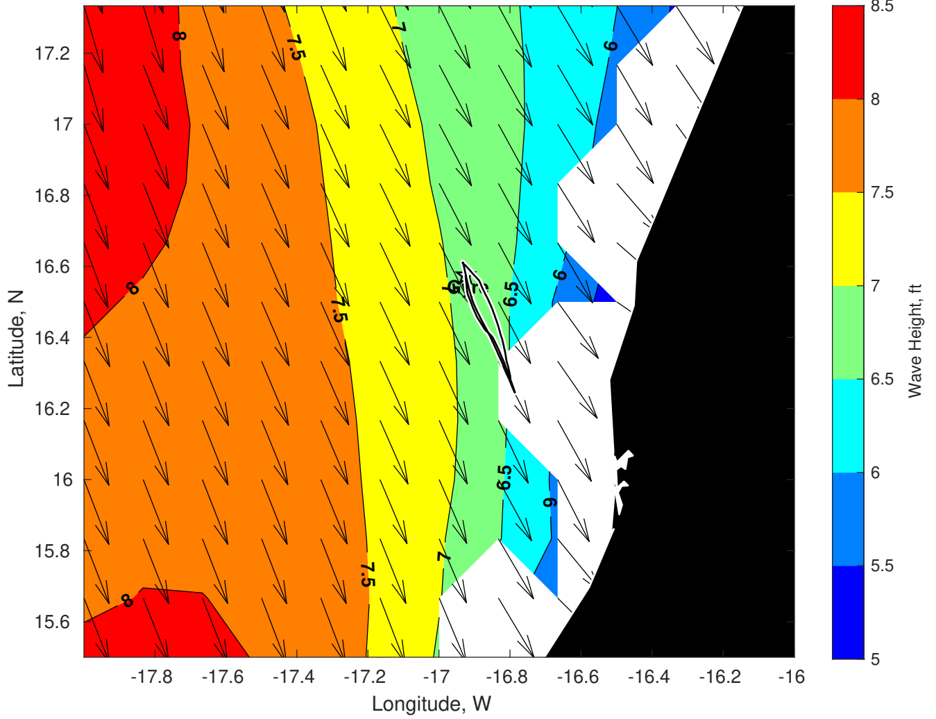
Wave Height (ft) for Gyre at 23-Mar-2025 09:00:00
