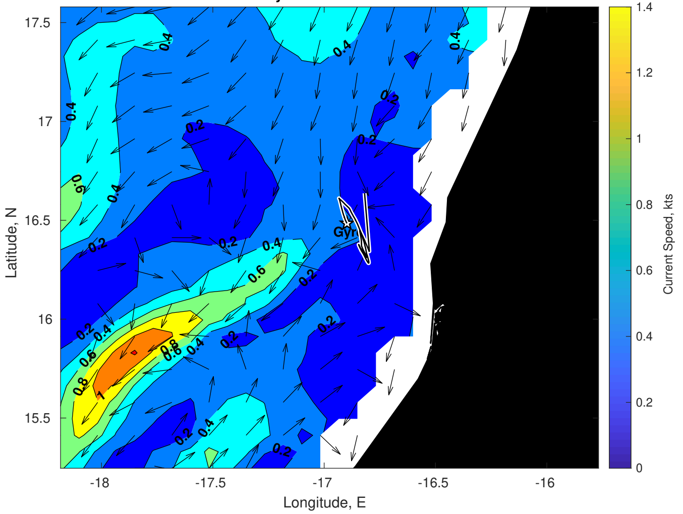
Surface Currents for Gyre at 22-Mar-2025 00:00:00
