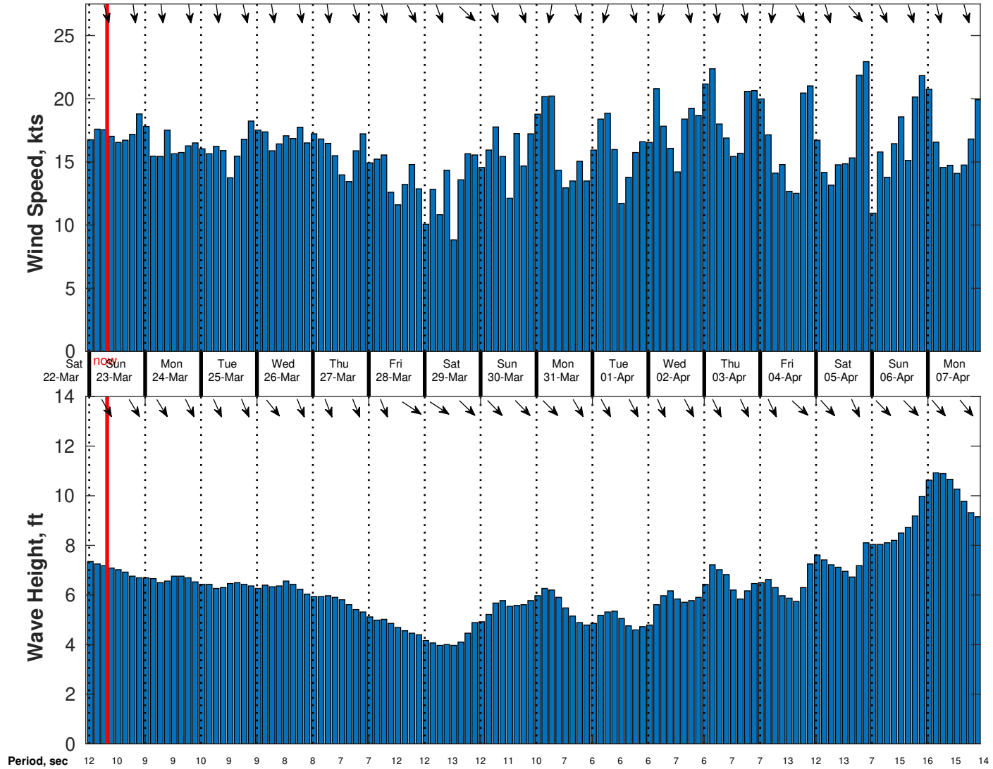
Wind & Wave Forecast for Gyre from 22-Mar-2025 23:00:00 to 07-Apr-2025 23:00:00
