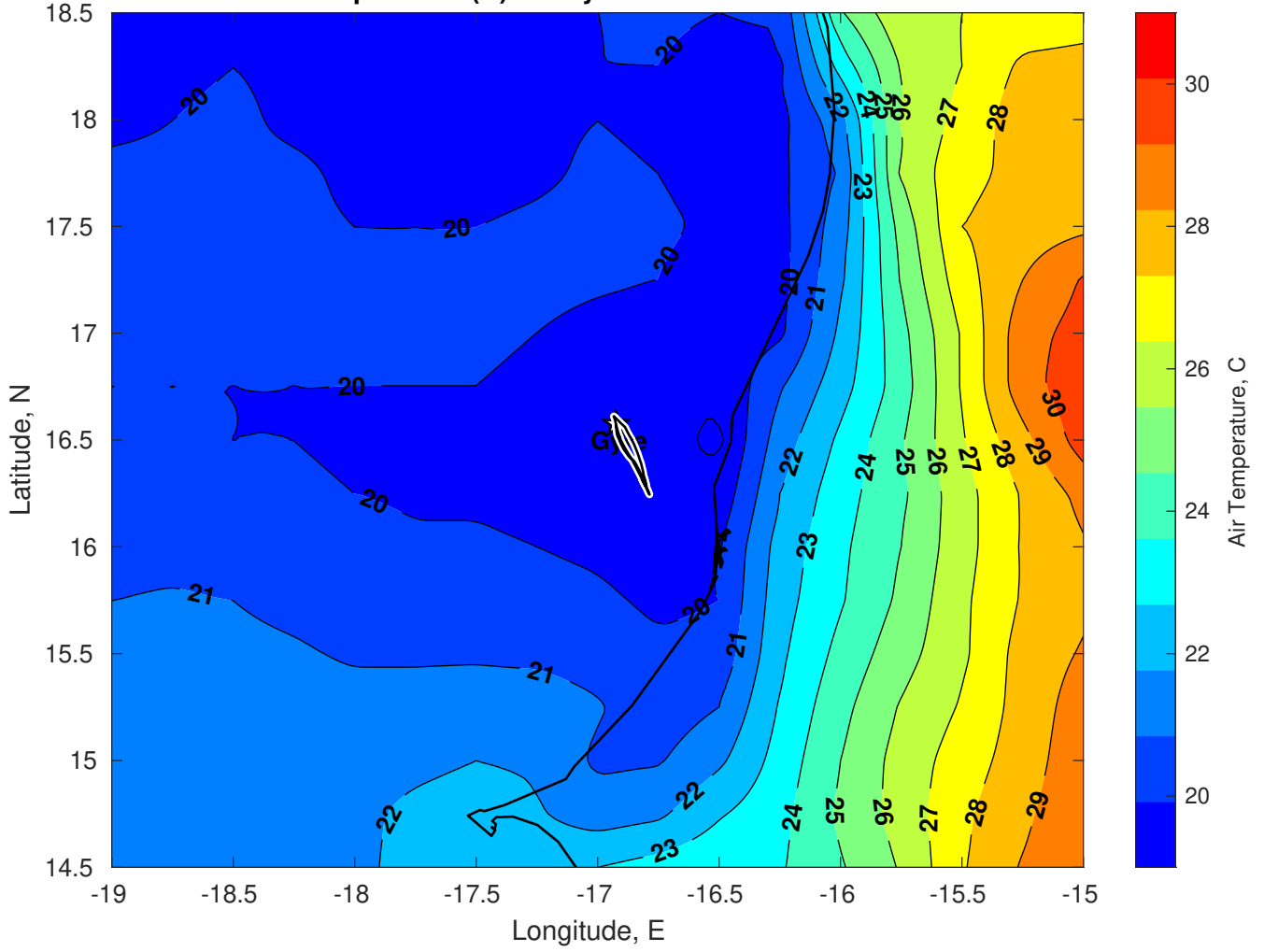
Air Temperature (C) for Gyre at 23-Mar-2025
