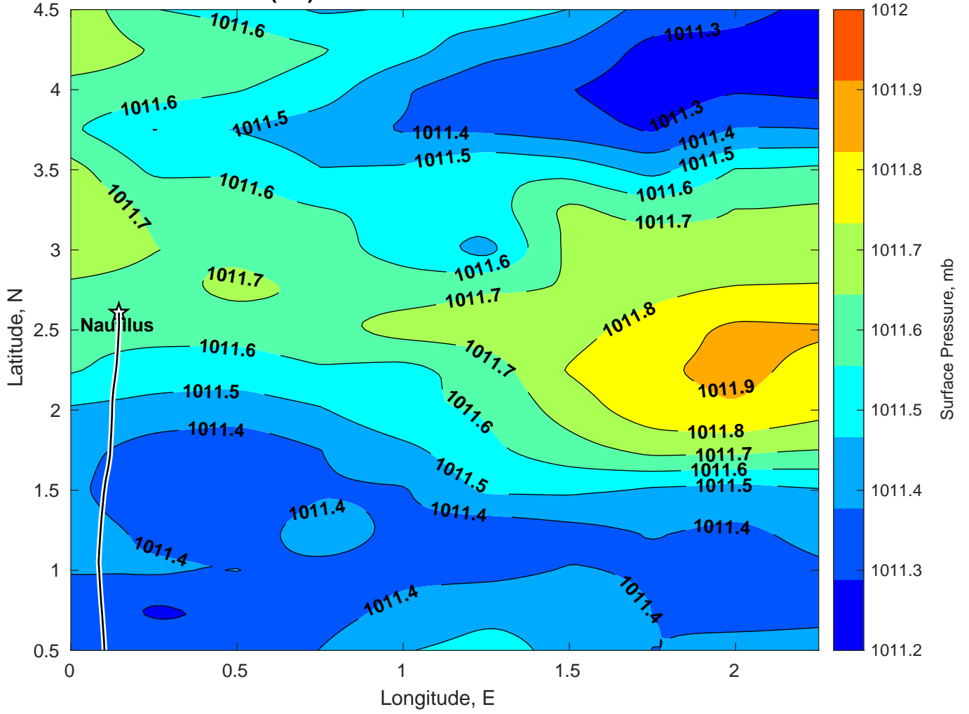
Surface Pressure (mb) for Nautilus at 23-Mar-2025 00:00:00
