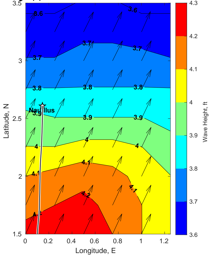
Wave Height (ft) for Nautilus at 23-Mar-2025 09:00:00
