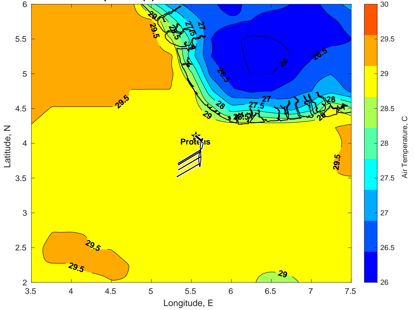
Air Temperature (C) for Proteus at 23-Mar-2025
