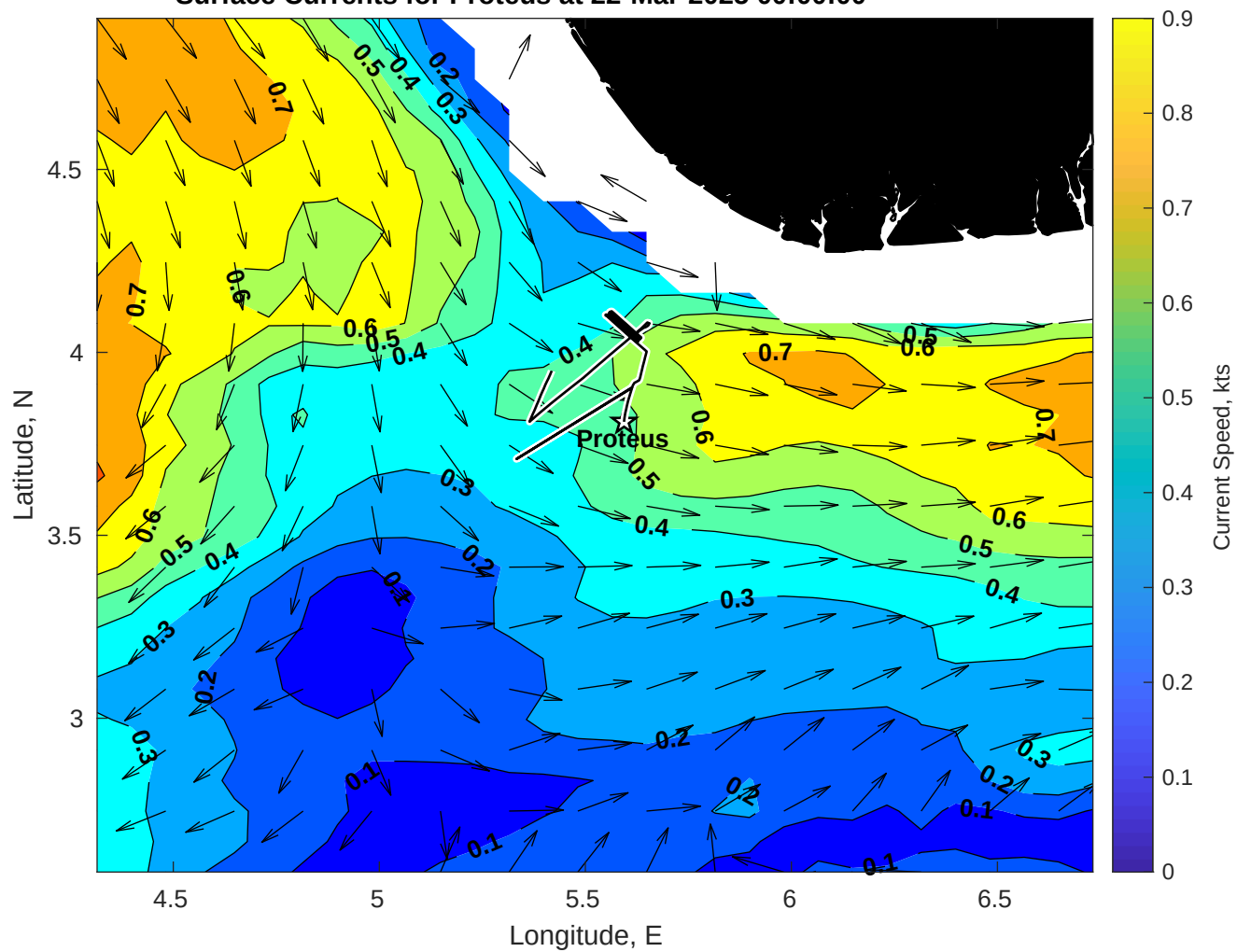
Surface Currents for Proteus at 22-Mar-2025 00:00:00
