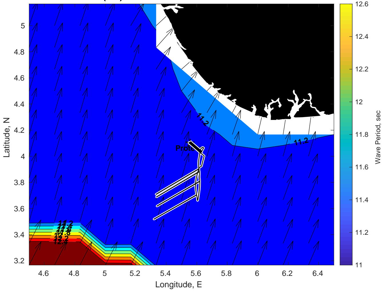
Wave Period (sec) for Proteus at 23-Mar-2025 09:00:00
