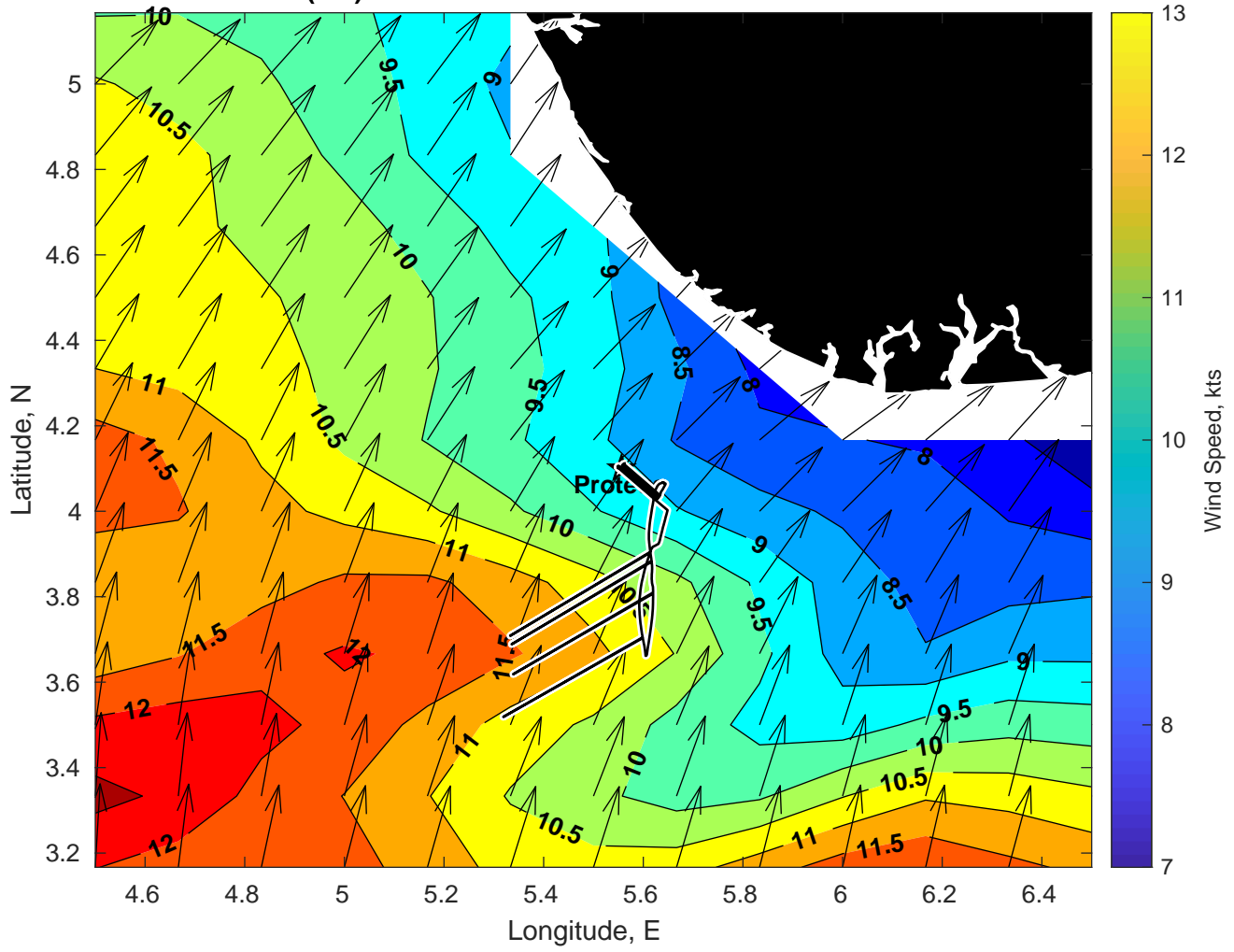
Winds (kts) for Proteus at 23-Mar-2025 09:00:00
