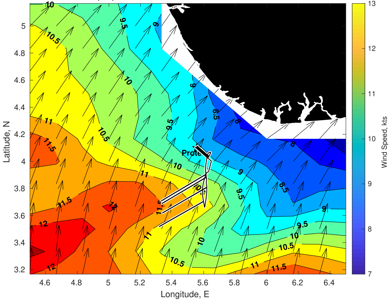
Winds (kts) for Proteus at 23-Mar-2025 09:00:00
