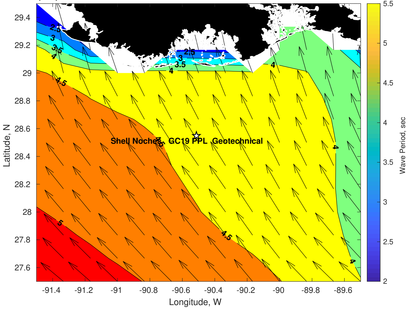
Wave Period (sec) for Shell Noches GC19 PPL Geotechnical at 23-Mar-2025 09:00:00
