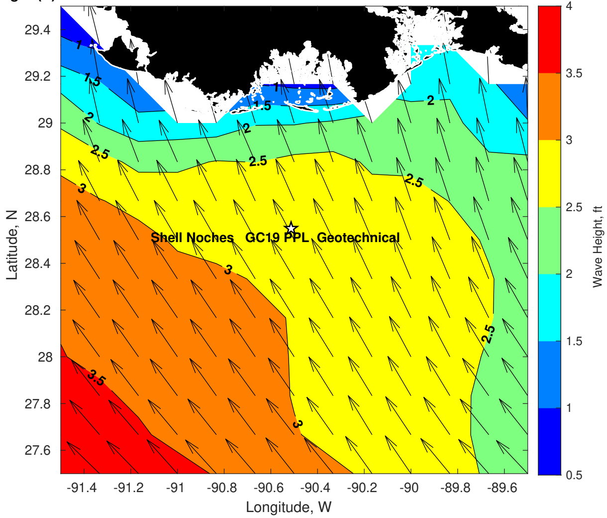
Wave Height (ft) for Shell Noches GC19 PPL Geotechnical at 23-Mar-2025 09:00:00
