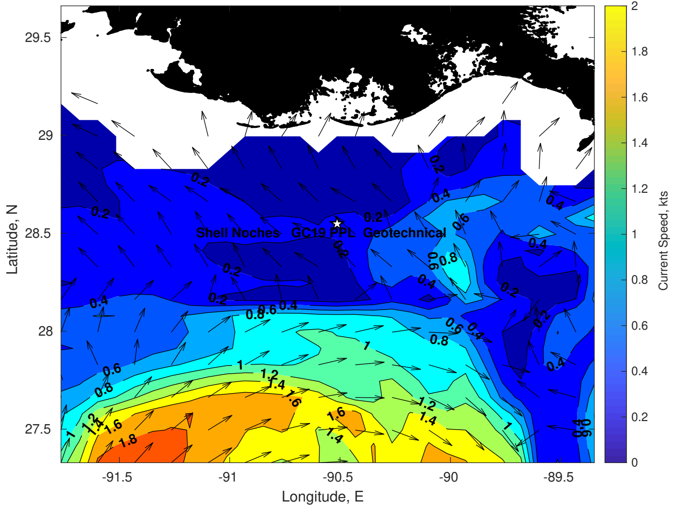
Surface Currents for Shell Noches GC19 PPL Geotechnical at 22-Mar-2025 00:00:00
