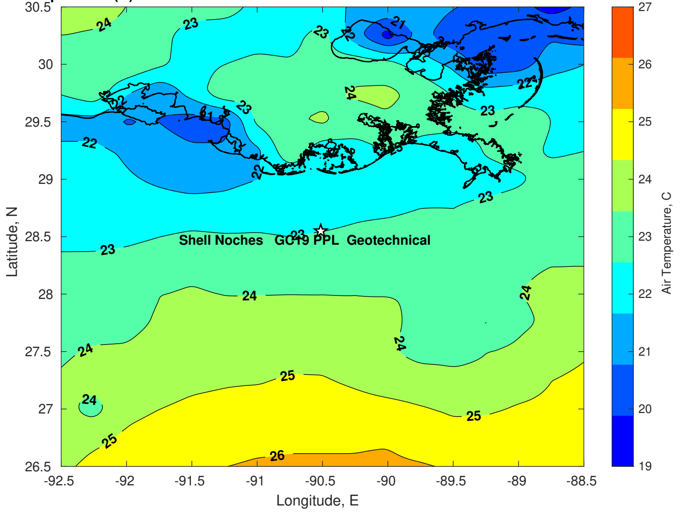
Air Temperature (C) for Shell Noches GC19 PPL Geotechnical at 23-Mar-2025
