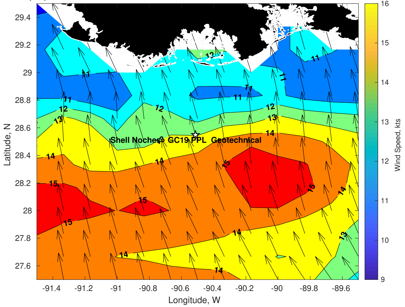
Winds (kts) for Shell Noches GC19 PPL Geotechnical at 23-Mar-2025 09:00:00
