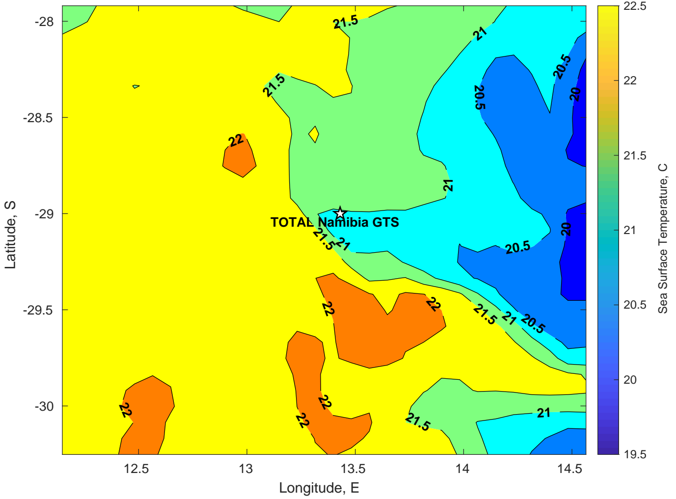
SST for TOTAL Namibia GTS at 22-Mar-2025 00:00:00
