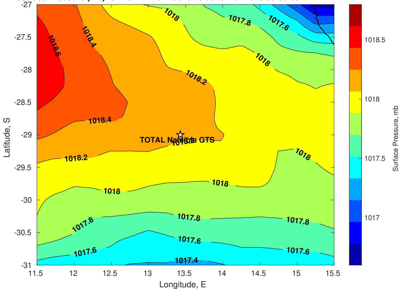
Surface Pressure (mb) for TOTAL Namibia GTS at 25-Mar-2025 00:00:00
