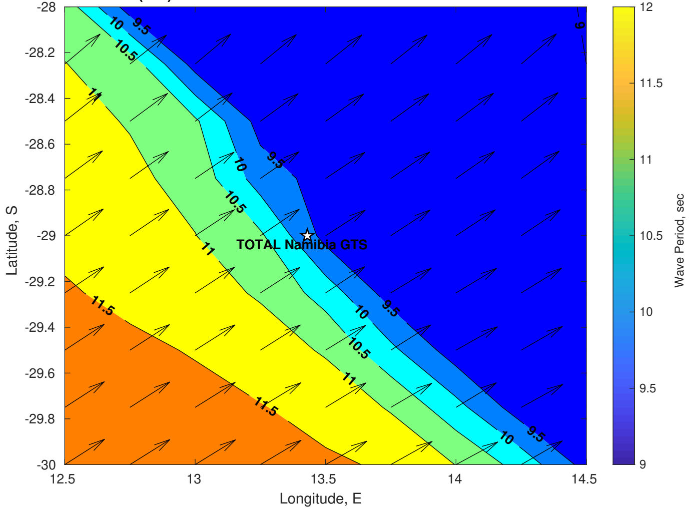
Wave Period (sec) for TOTAL Namibia GTS at 23-Mar-2025 09:00:00
