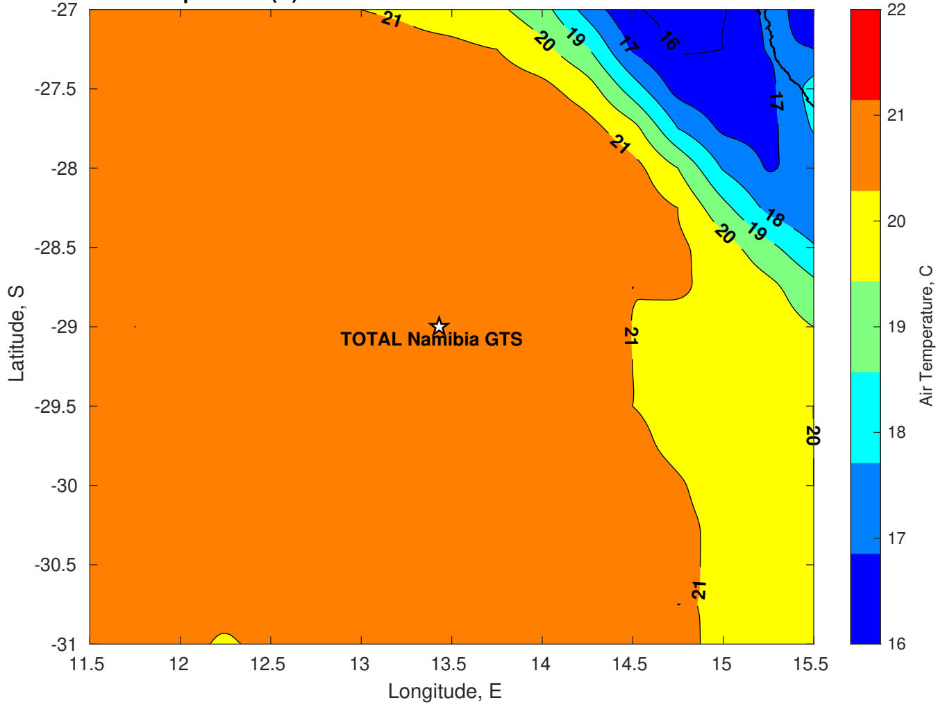
Air Temperature (C) for TOTAL Namibia GTS at 23-Mar-2025
