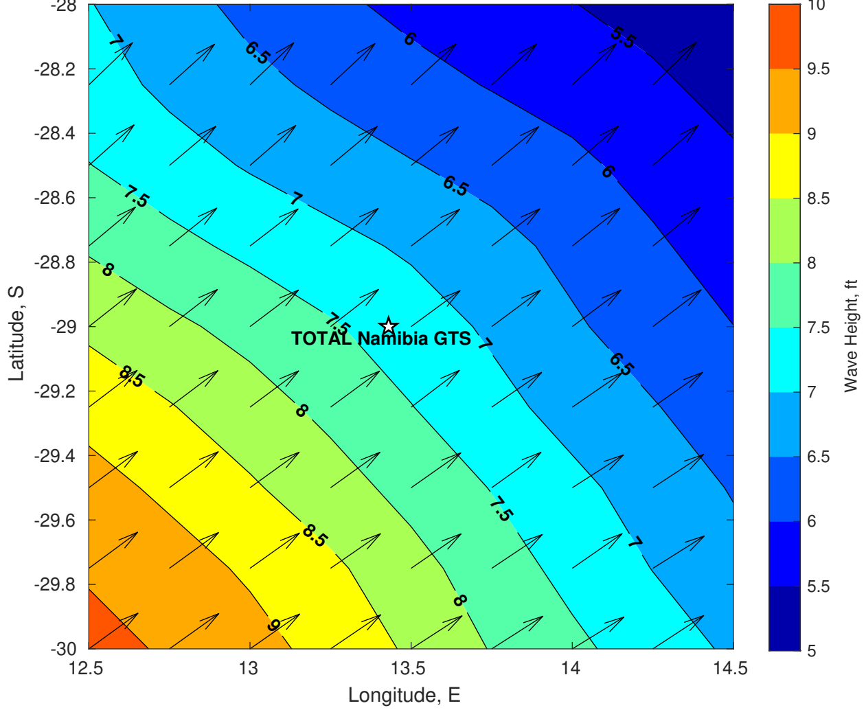
Wave Height (ft) for TOTAL Namibia GTS at 23-Mar-2025 09:00:00
