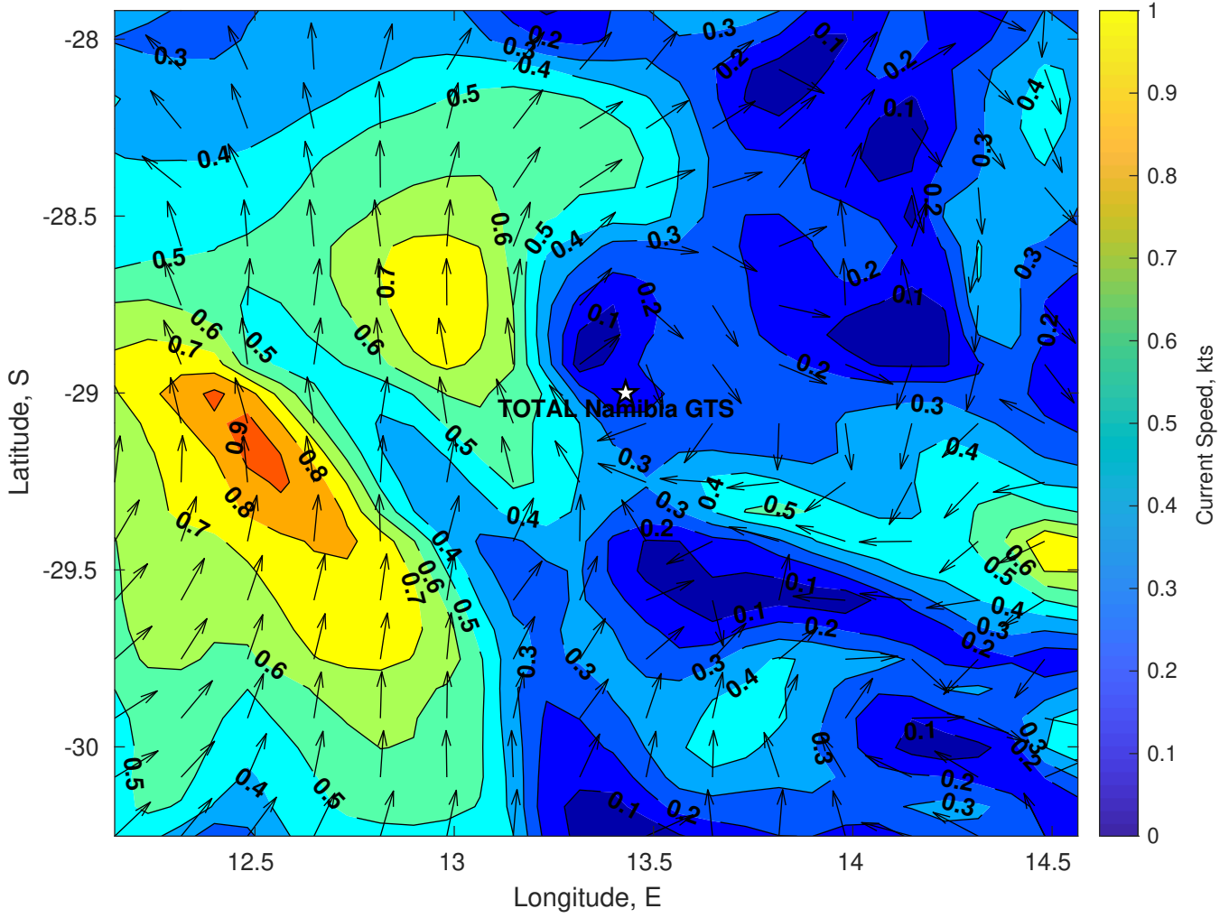
Surface Currents for TOTAL Namibia GTS at 22-Mar-2025 00:00:00
