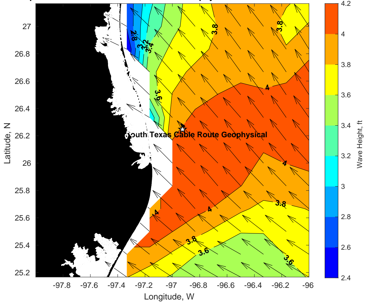
Wave Height (ft) for Tampnet P2378 South Texas Cable Route Geophysical at 23-Mar-2025 09:00:00
