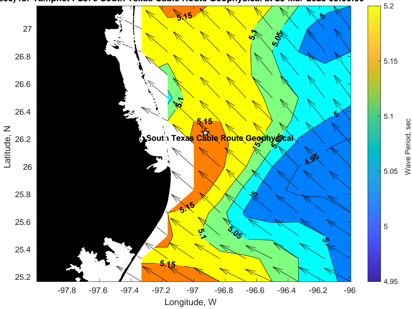
Period (sec) for Tampnet P2378 South Texas Cable Route Geophysical at 23-Mar-2025 09:00:00
