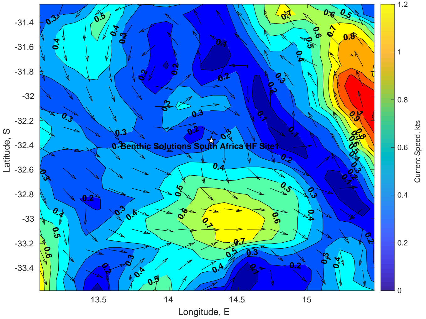
Surface Currents for Benthic Solutions South Africa HF Site1 at 23-Mar-2025 00:00:00
