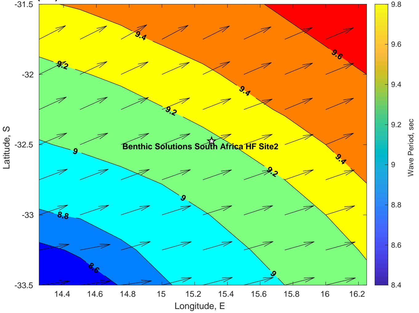
Wave Period (sec) for Benthic Solutions South Africa HF Site2 at 24-Mar-2025 09:00:00
