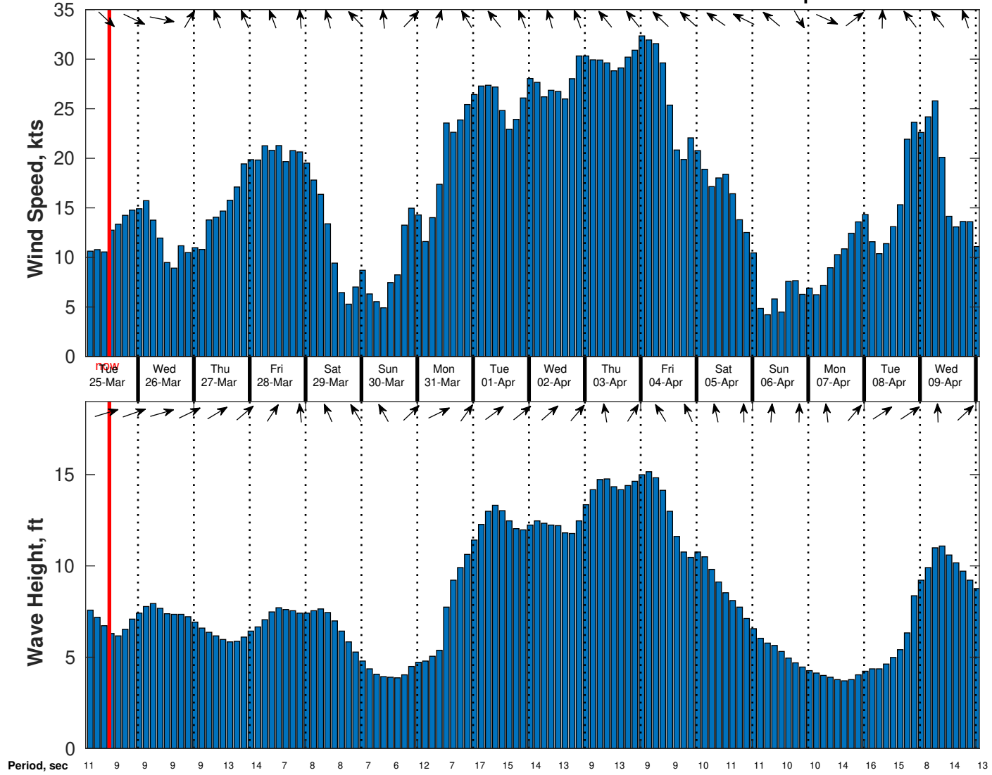
Wind & Wave Forecast for Benthic Solutions South Africa HF Site3 from 24-Mar-2025 02:00:00 to 09-Apr-2025 02:00:00
