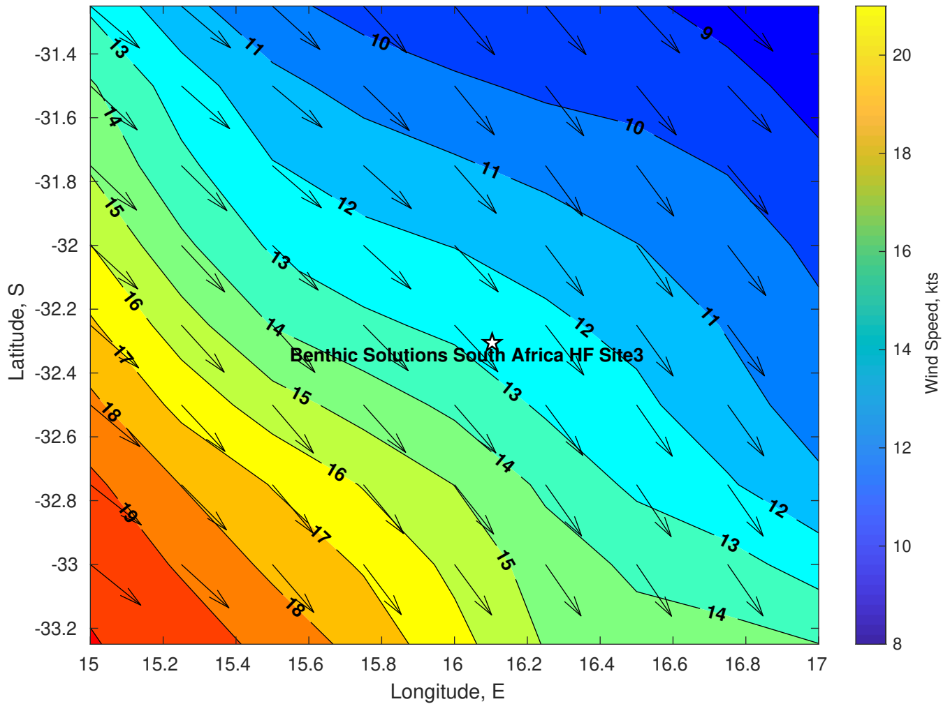
Winds (kts) for Benthic Solutions South Africa HF Site3 at 24-Mar-2025 09:00:00
