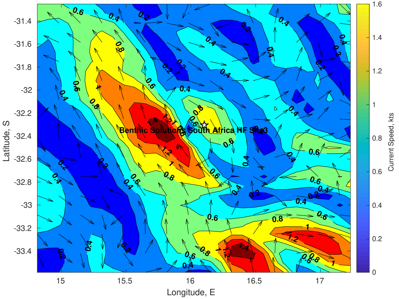
Surface Currents for Benthic Solutions South Africa HF Site3 at 23-Mar-2025 00:00:00
