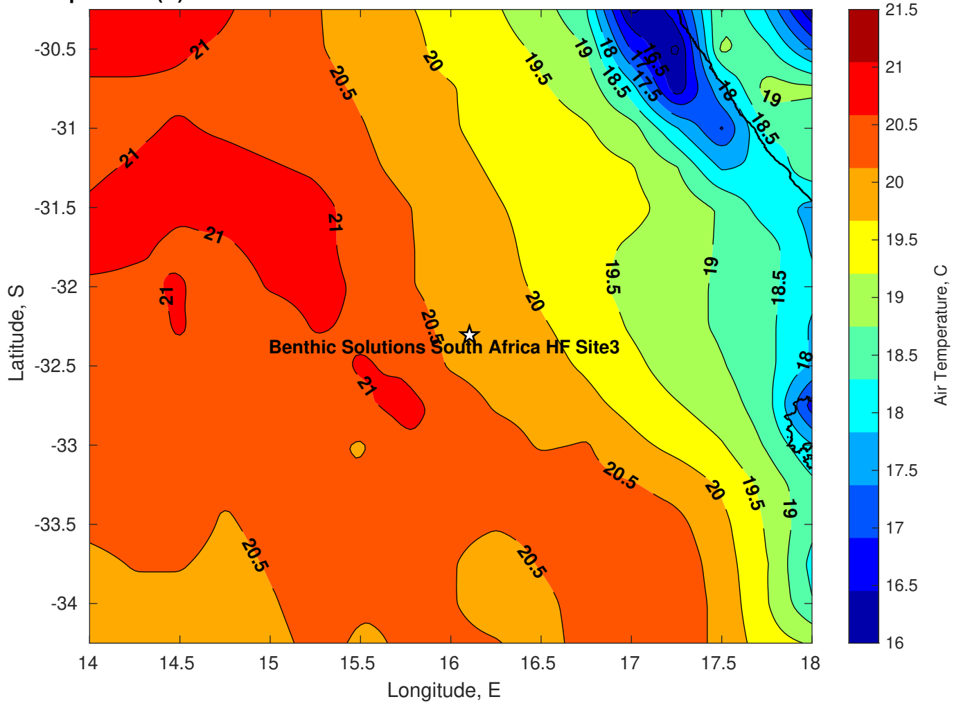
Air Temperature (C) for Benthic Solutions South Africa HF Site3 at 24-Mar-2025
