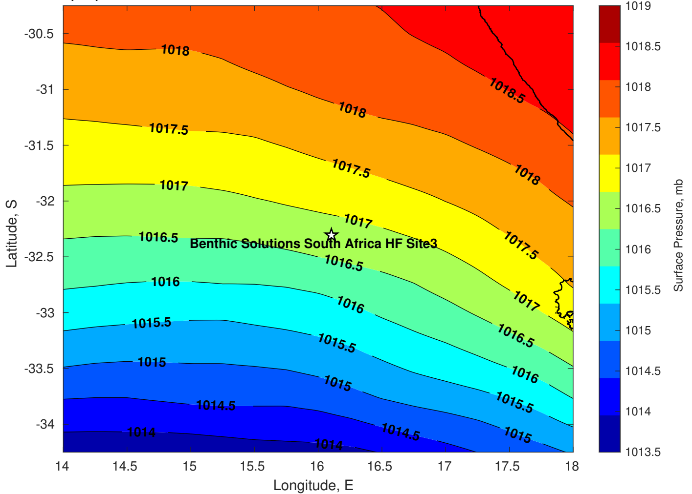
Surface Pressure (mb) for Benthic Solutions South Africa HF Site3 at 25-Mar-2025 00:00:00
