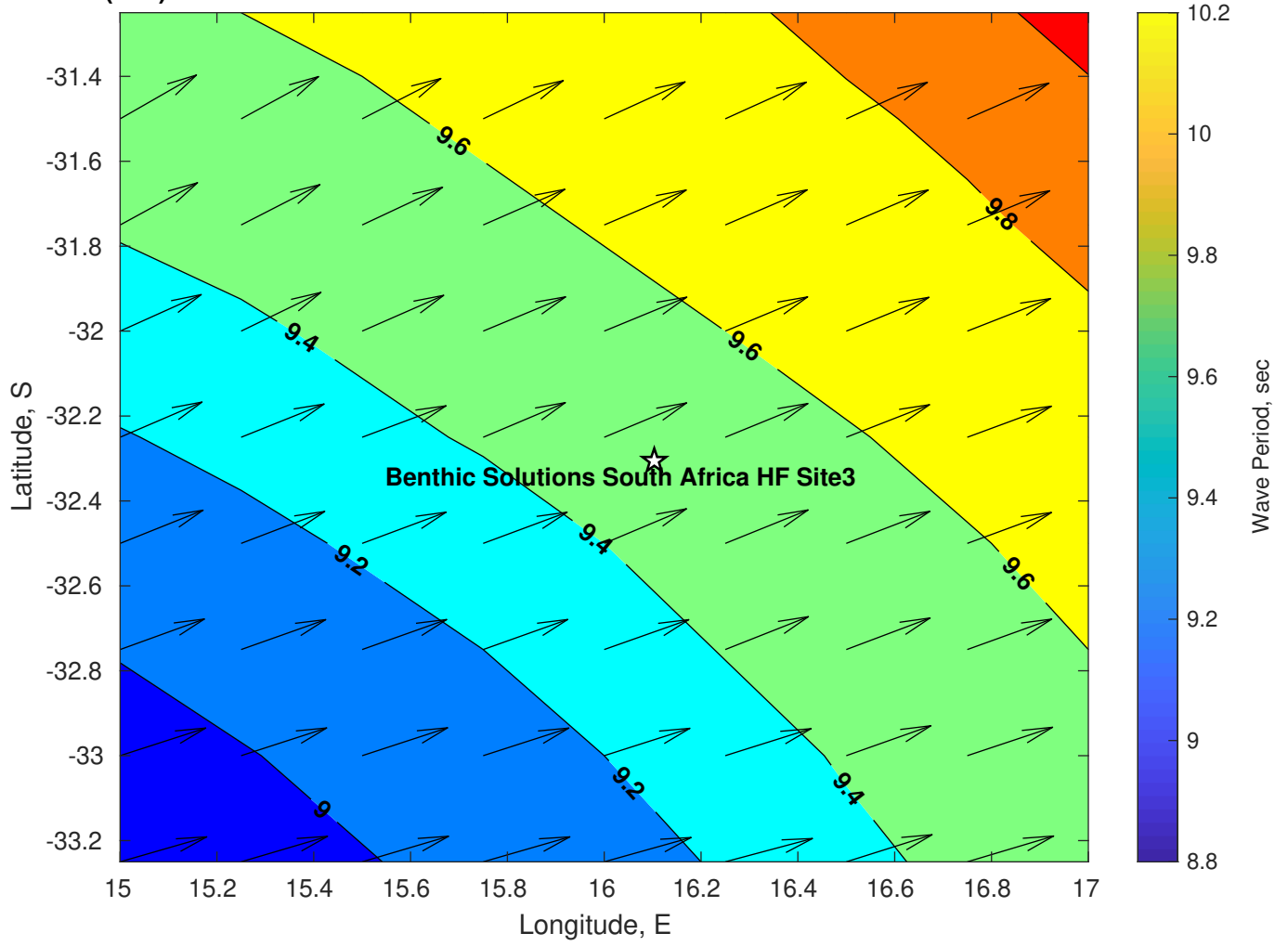
Wave Period (sec) for Benthic Solutions South Africa HF Site3 at 24-Mar-2025 09:00:00
