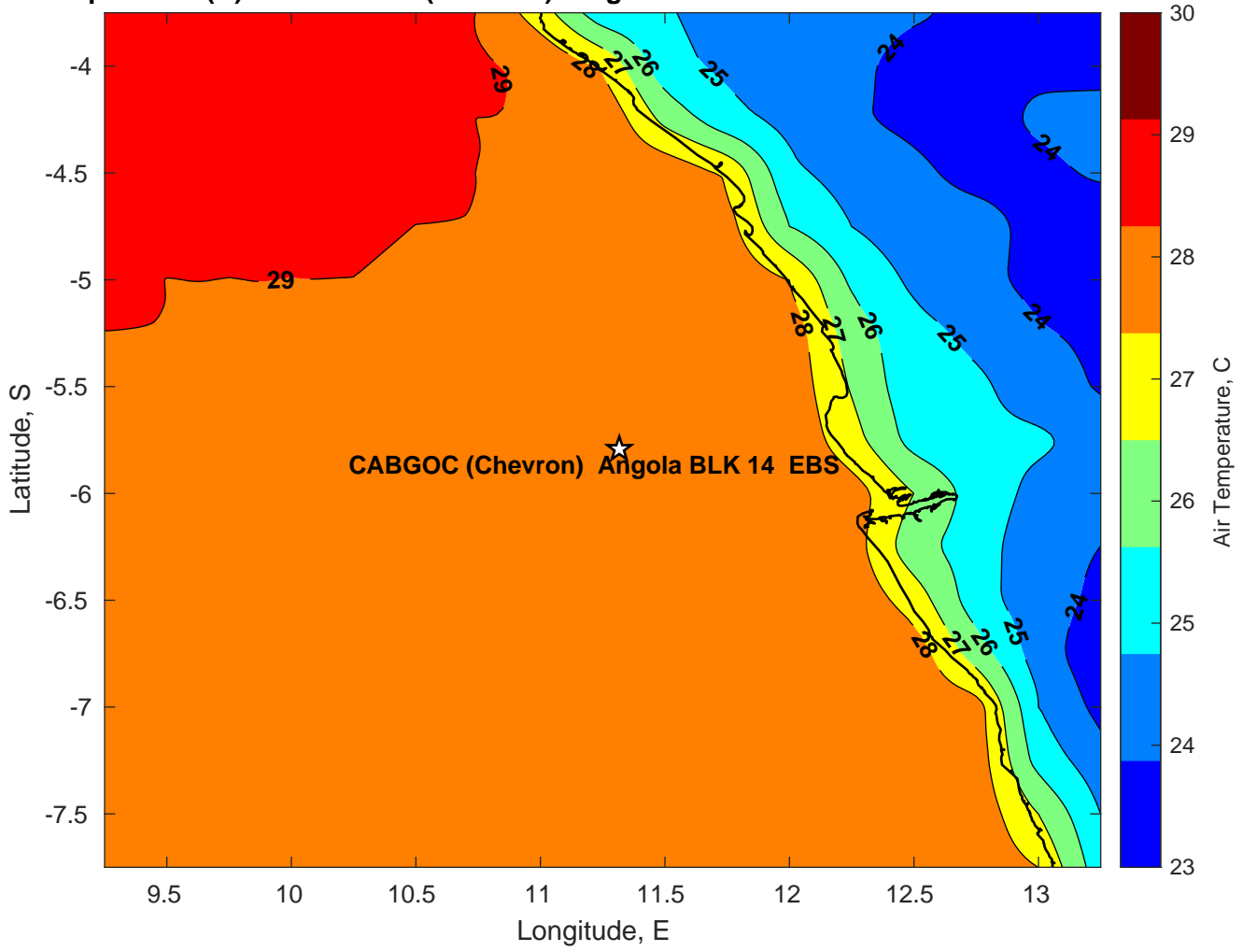
Air Temperature (C) for CABGOC (Chevron) Angola BLK 14 EBS at 24-Mar-2025
