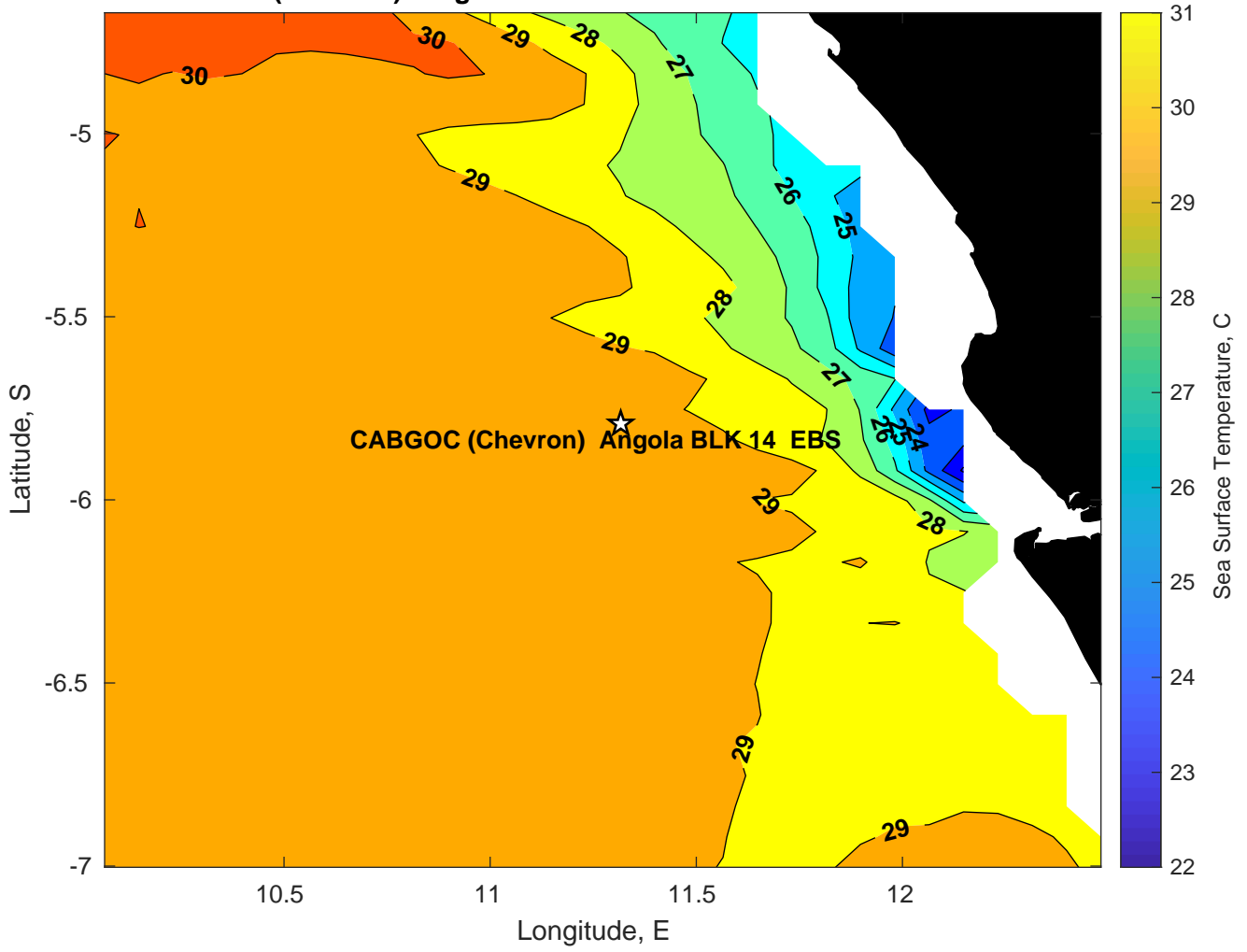
SST for CABGOC (Chevron) Angola BLK 14 EBS at 23-Mar-2025 00:00:00
