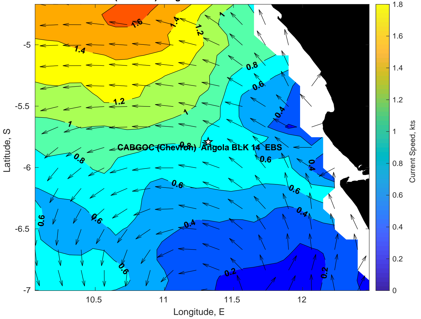
Surface Currents for CABGOC (Chevron) Angola BLK 14 EBS at 23-Mar-2025 00:00:00
