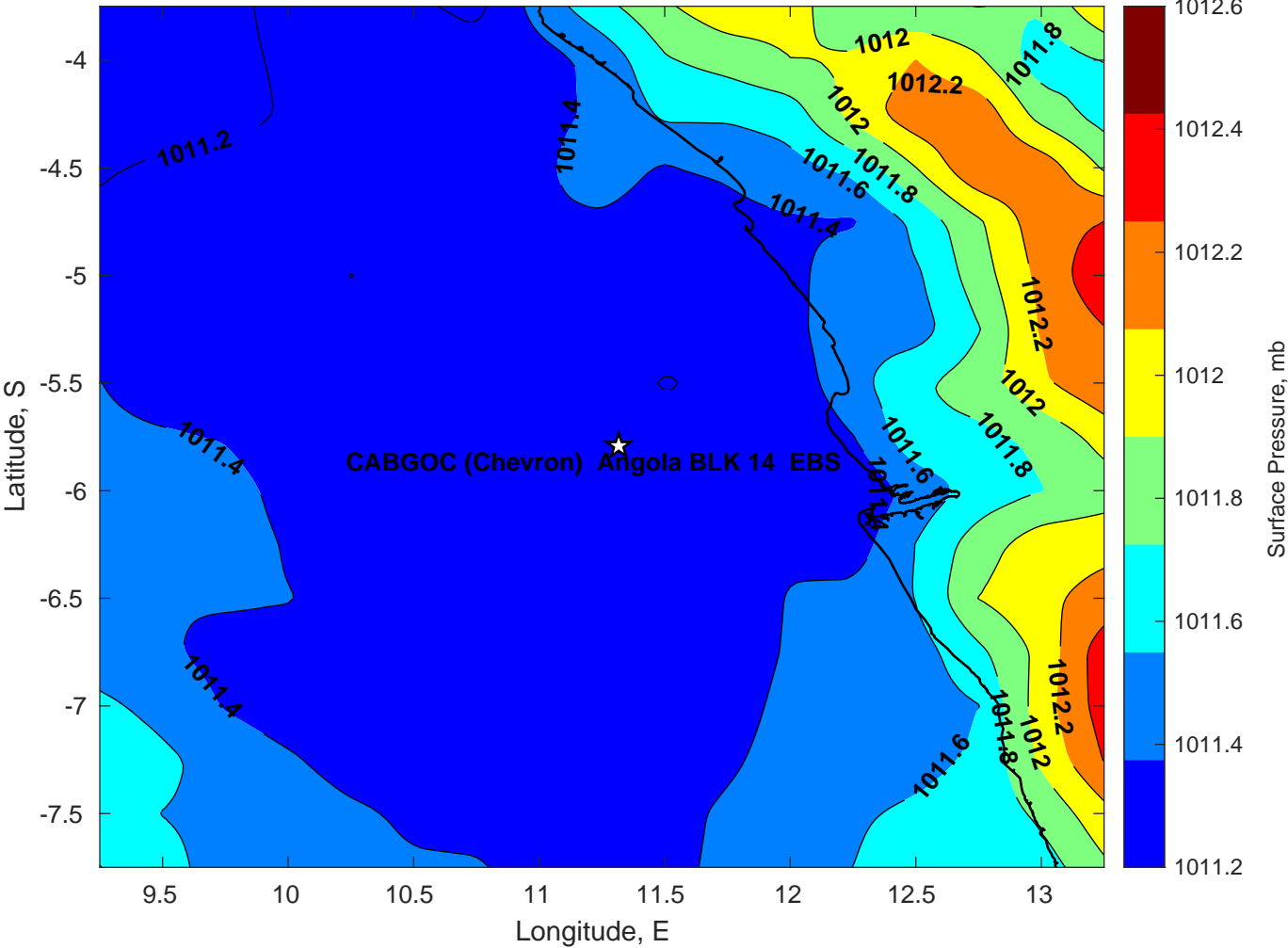
Surface Pressure (mb) for CABGOC (Chevron) Angola BLK 14 EBS at 24-Mar-2025 00:00:00
