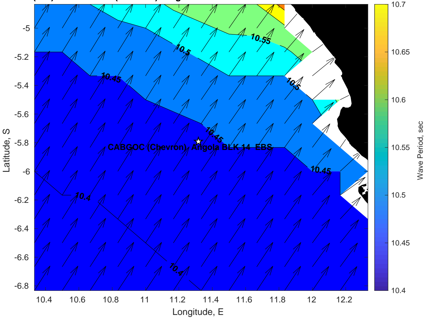
Wave Period (sec) for CABGOC (Chevron) Angola BLK 14 EBS at 24-Mar-2025 09:00:00
