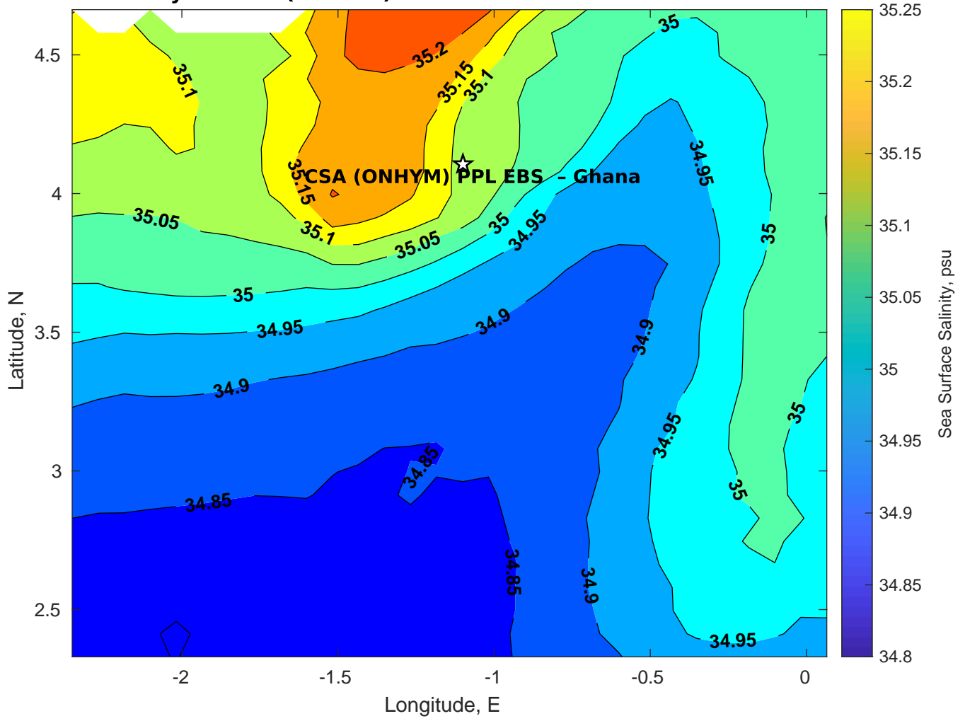
Surface Salinity for CSA (ONHYM) PPL EBS - Ghana at 23-Mar-2025 00:00:00
