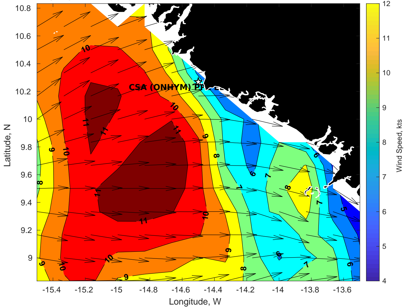
Winds (kts) for CSA (ONHYM) PPL EBS - Guinea at 24-Mar-2025 09:00:00
