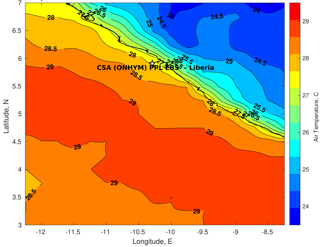
Air Temperature (C) for CSA (ONHYM) PPL EBS - Liberia at 24-Mar-2025
