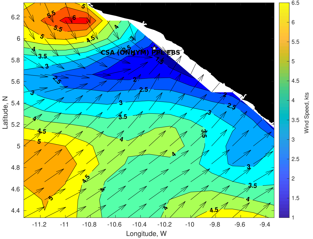
Winds (kts) for CSA (ONHYM) PPL EBS - Liberia at 24-Mar-2025 09:00:00
