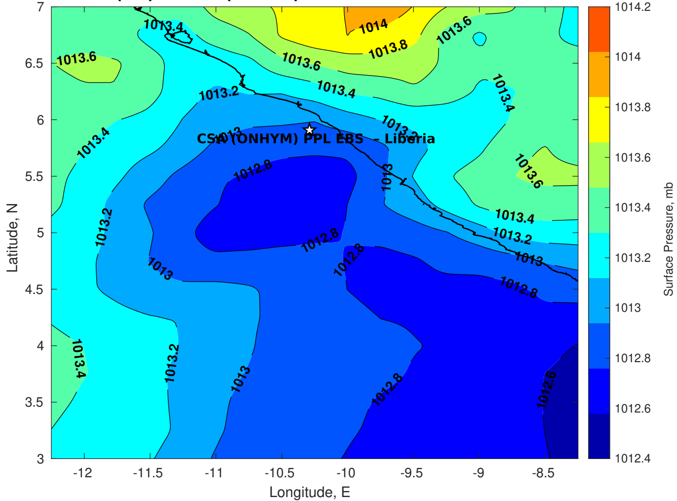
Surface Pressure (mb) for CSA (ONHYM) PPL EBS - Liberia at 25-Mar-2025 00:00:00
