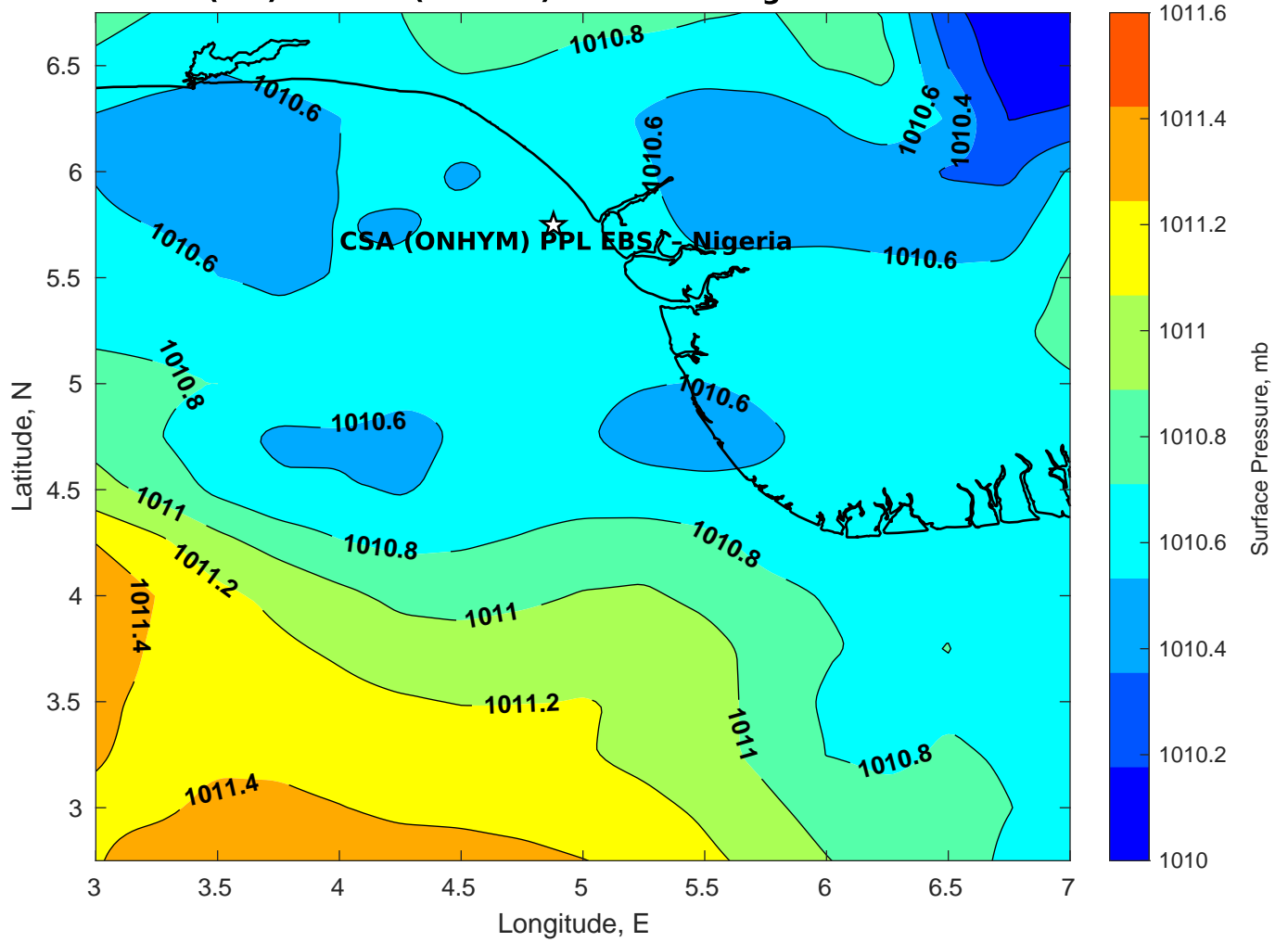
Surface Pressure (mb) for CSA (ONHYM) PPL EBS - Nigeria at 24-Mar-2025 00:00:00
