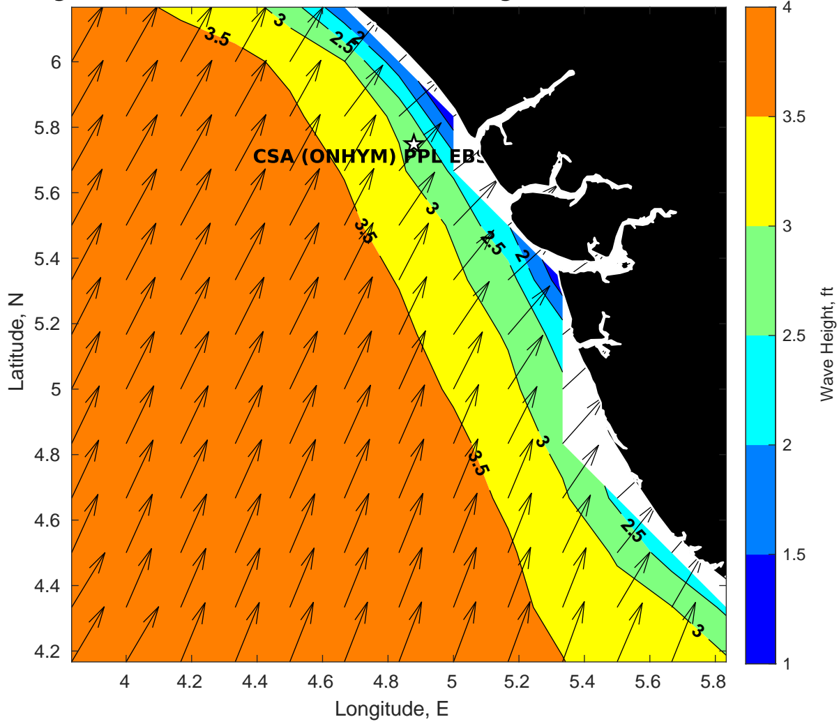
Wave Height (ft) for CSA (ONHYM) PPL EBS - Nigeria at 24-Mar-2025 09:00:00
