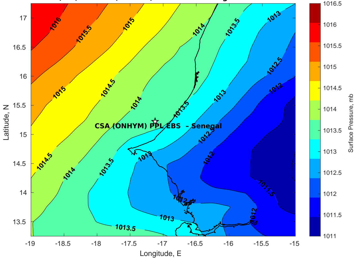
Surface Pressure (mb) for CSA (ONHYM) PPL EBS - Senegal at 25-Mar-2025 00:00:00
