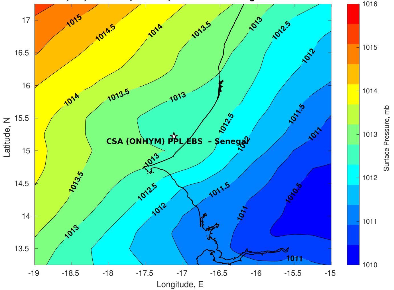
Surface Pressure (mb) for CSA (ONHYM) PPL EBS - Senegal at 24-Mar-2025 00:00:00
