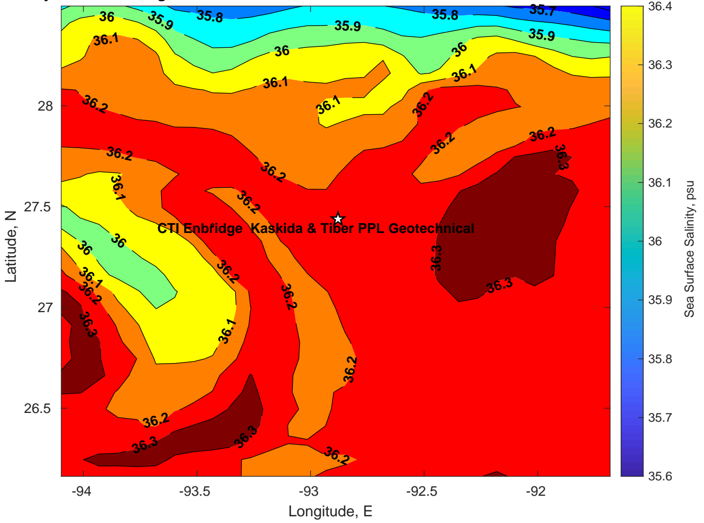
Surface Salinity for CTI Enbridge Kaskida & Tiber PPL Geotechnical at 23-Mar-2025 00:00:00
