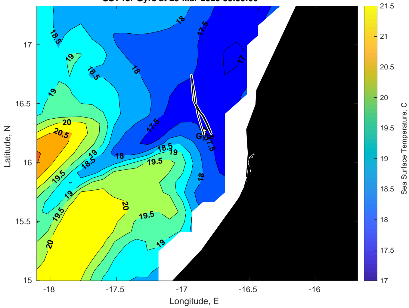
SST for Gyre at 23-Mar-2025 00:00:00
