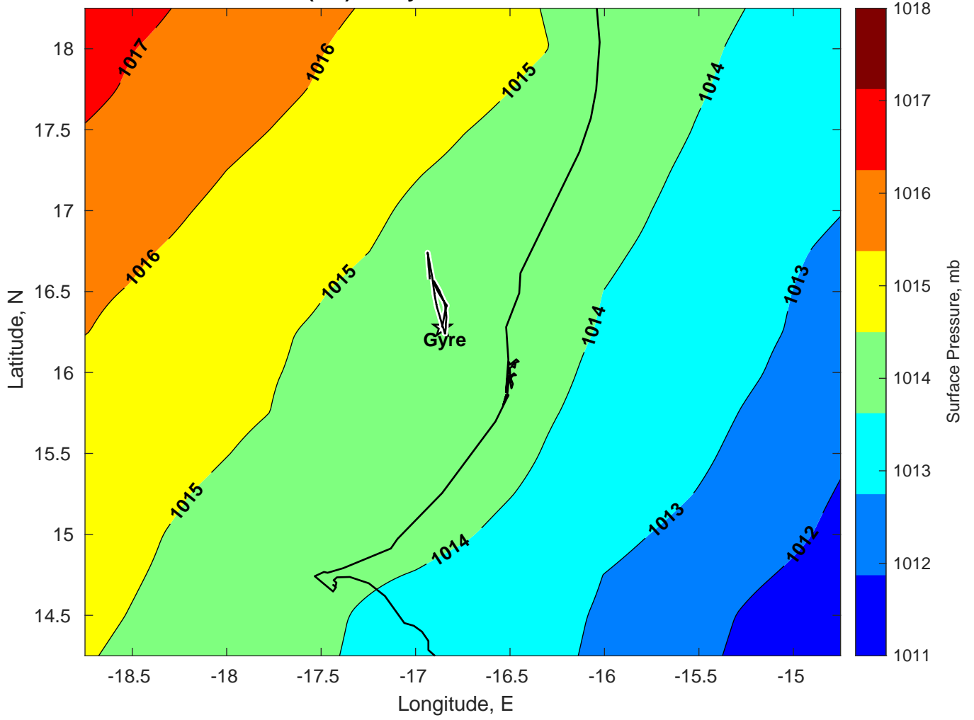
Surface Pressure (mb) for Gyre at 26-Mar-2025 00:00:00
