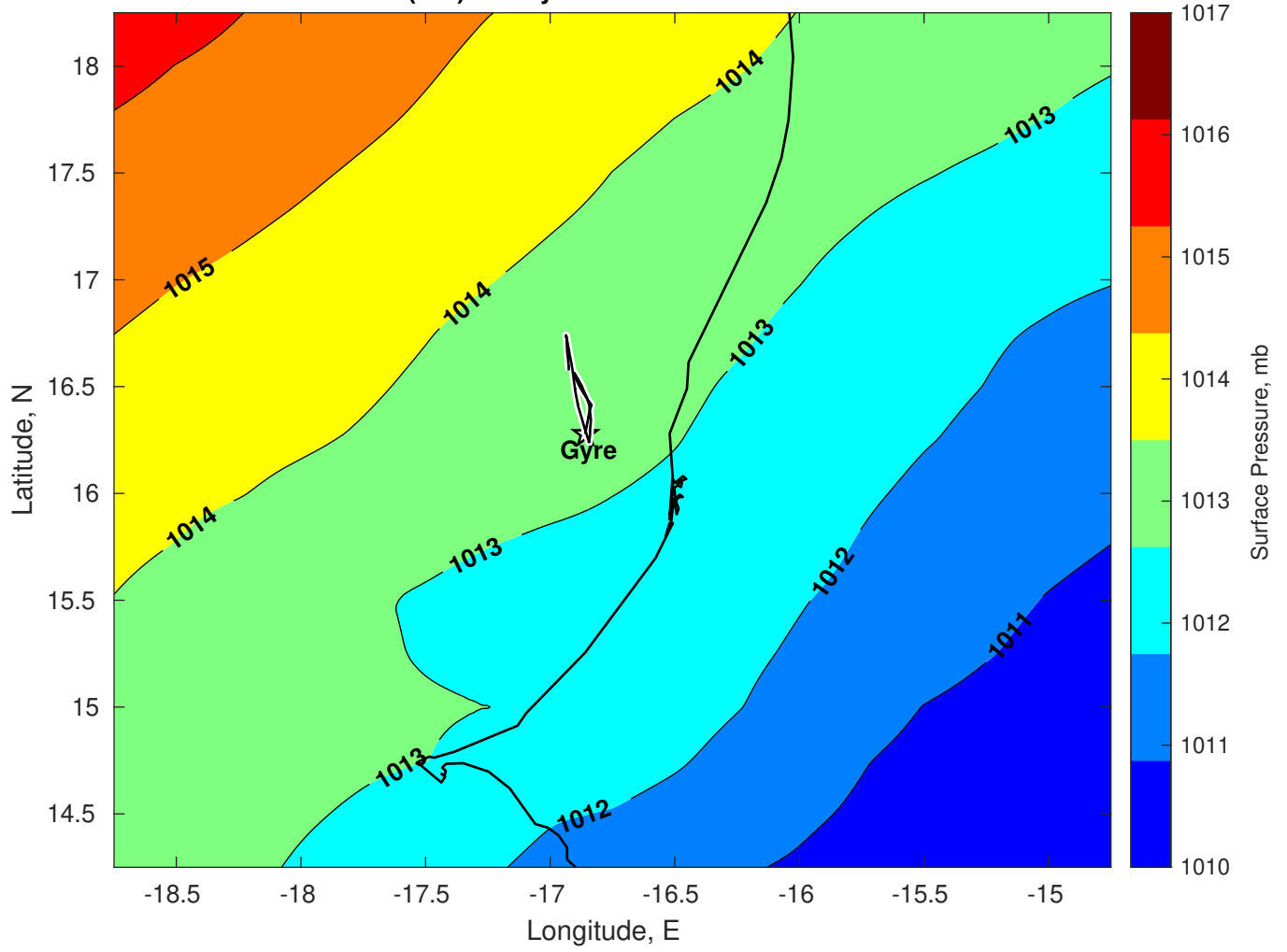
Surface Pressure (mb) for Gyre at 24-Mar-2025 00:00:00
