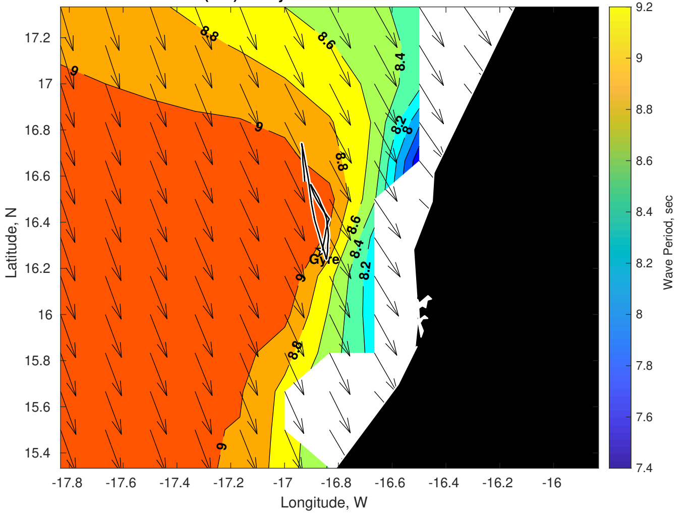
Wave Period (sec) for Gyre at 24-Mar-2025 09:00:00
