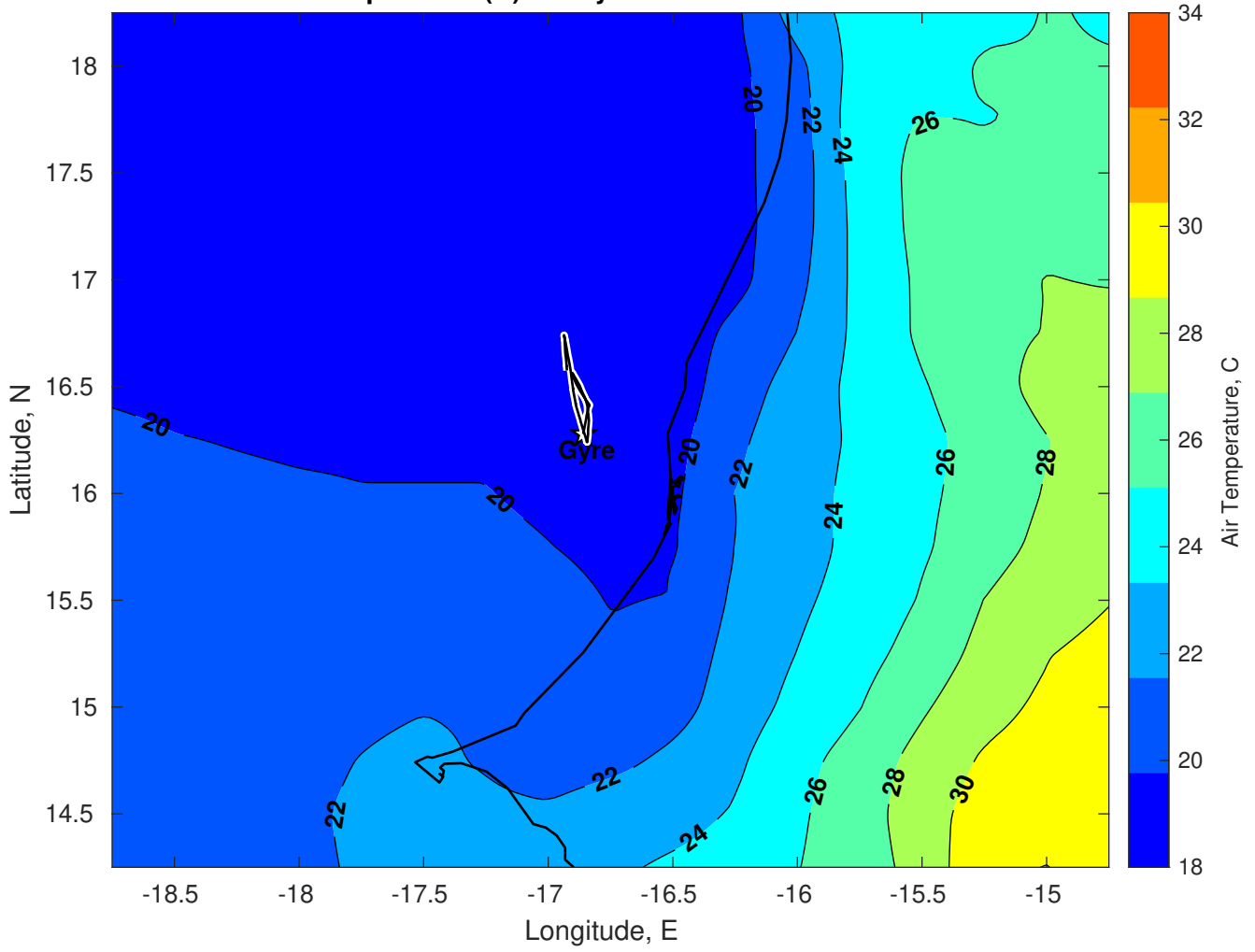
Air Temperature (C) for Gyre at 24-Mar-2025
