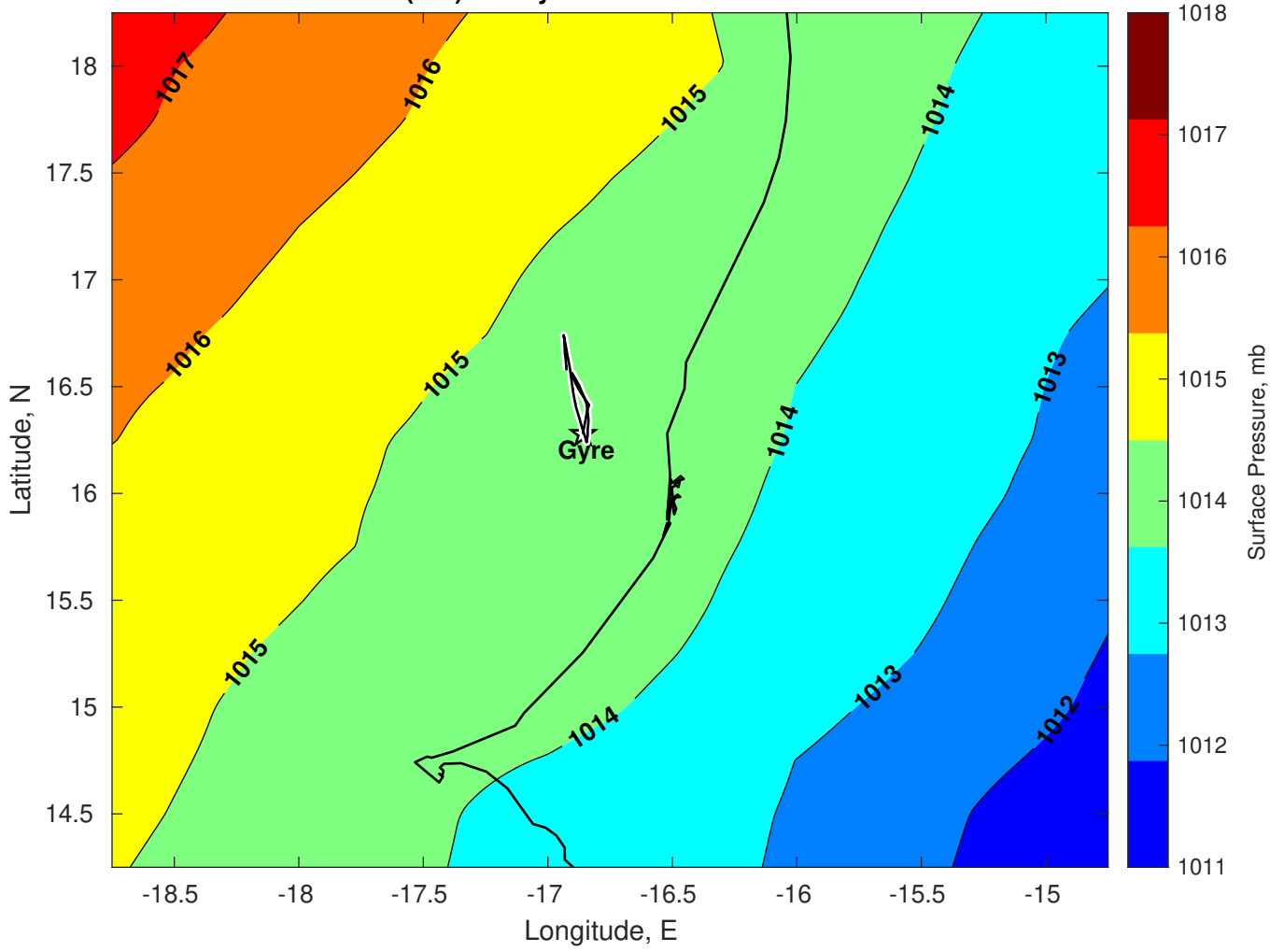
Surface Pressure (mb) for Gyre at 26-Mar-2025 00:00:00
