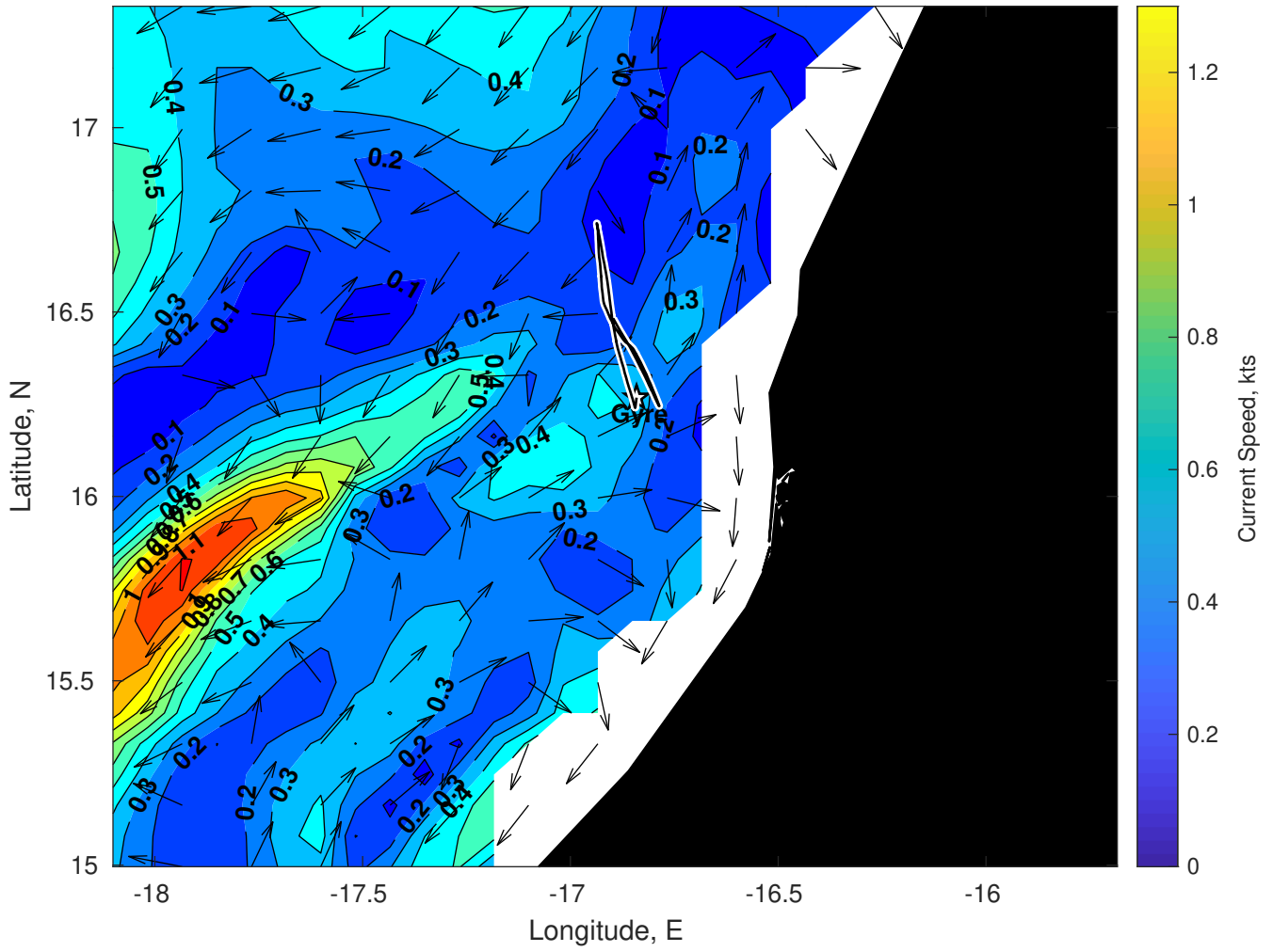
Surface Currents for Gyre at 23-Mar-2025 00:00:00
