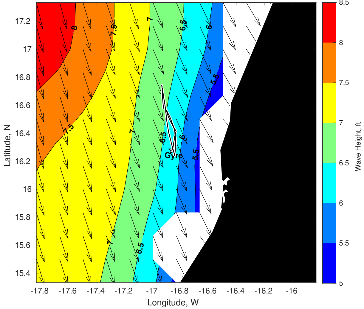
Wave Height (ft) for Gyre at 24-Mar-2025 09:00:00
