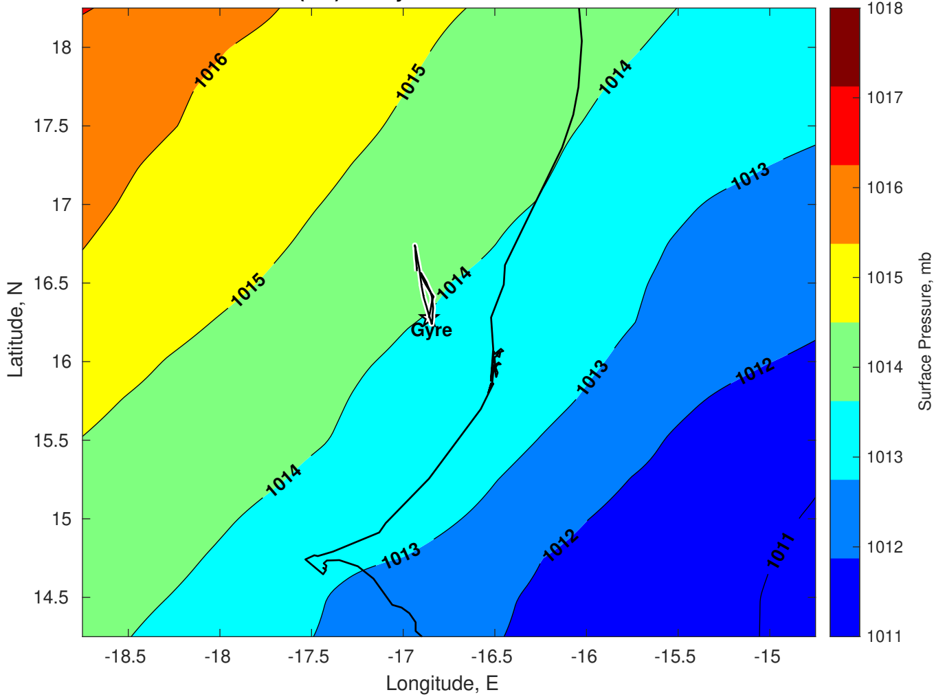
Surface Pressure (mb) for Gyre at 25-Mar-2025 00:00:00
