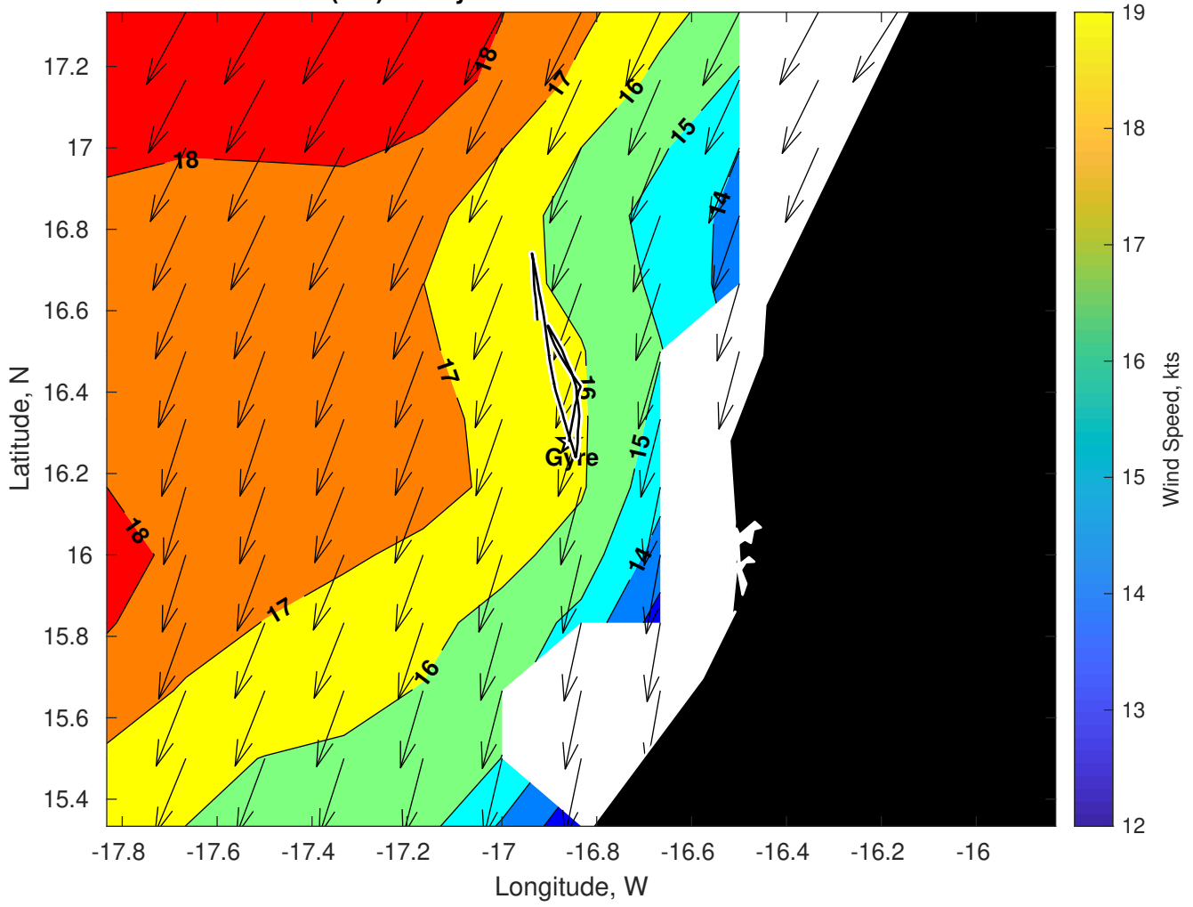
Winds (kts) for Gyre at 24-Mar-2025 09:00:00
