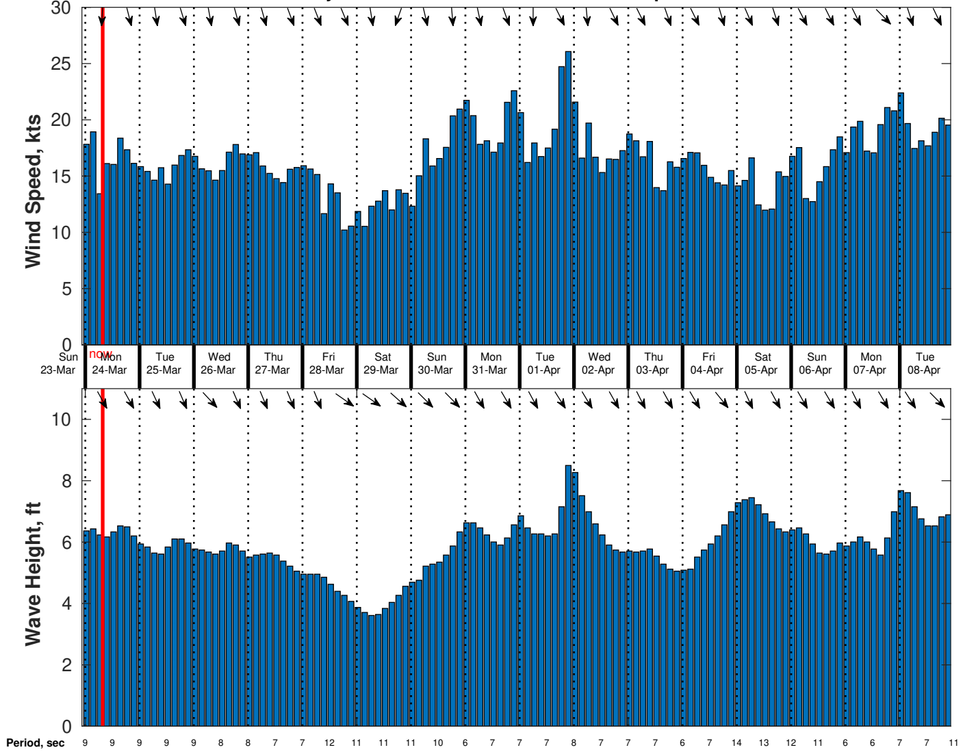
Wind & Wave Forecast for Gyre from 23-Mar-2025 23:00:00 to 08-Apr-2025 23:00:00
