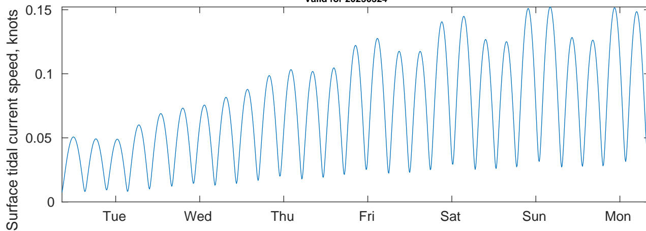
Tidal Currents and Heights for Gyre at 20250324
