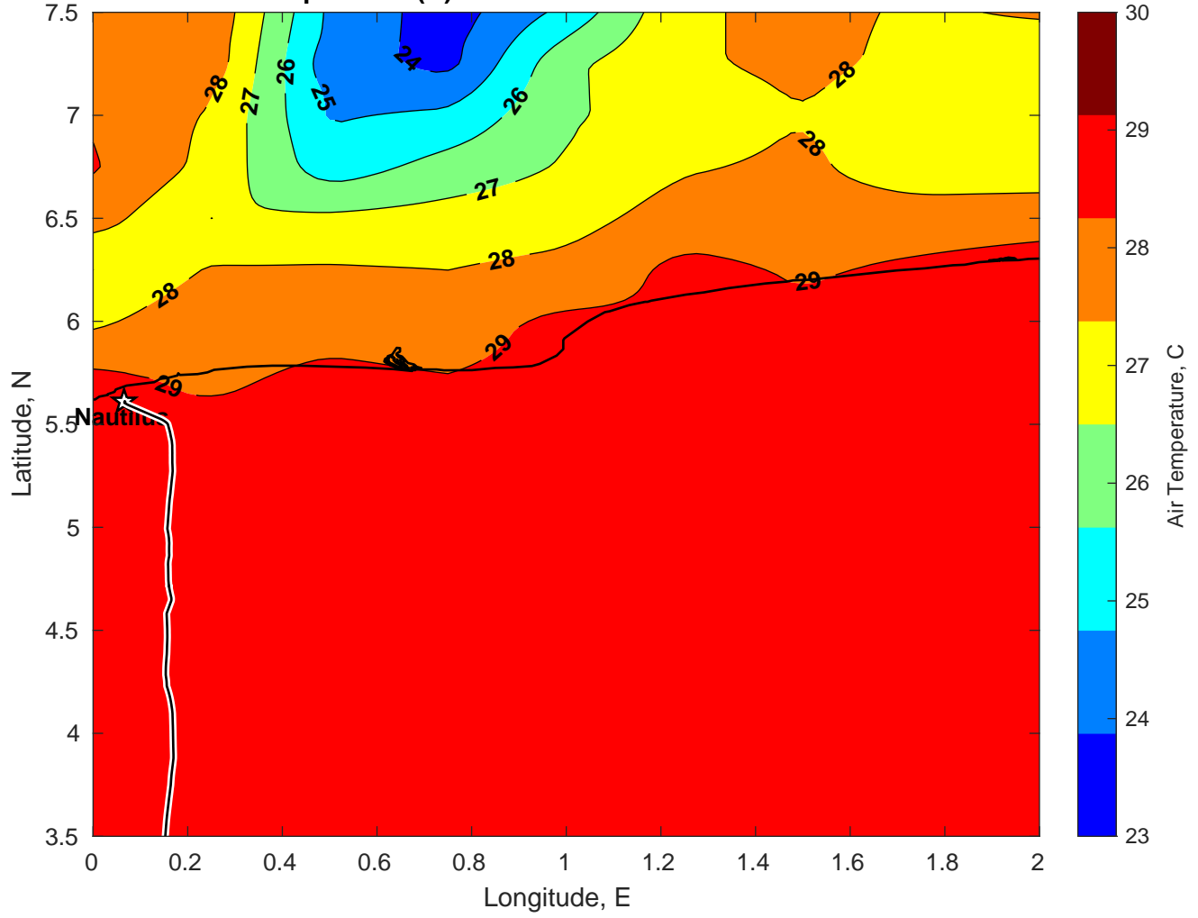
Air Temperature (C) for Nautilus at 24-Mar-2025
