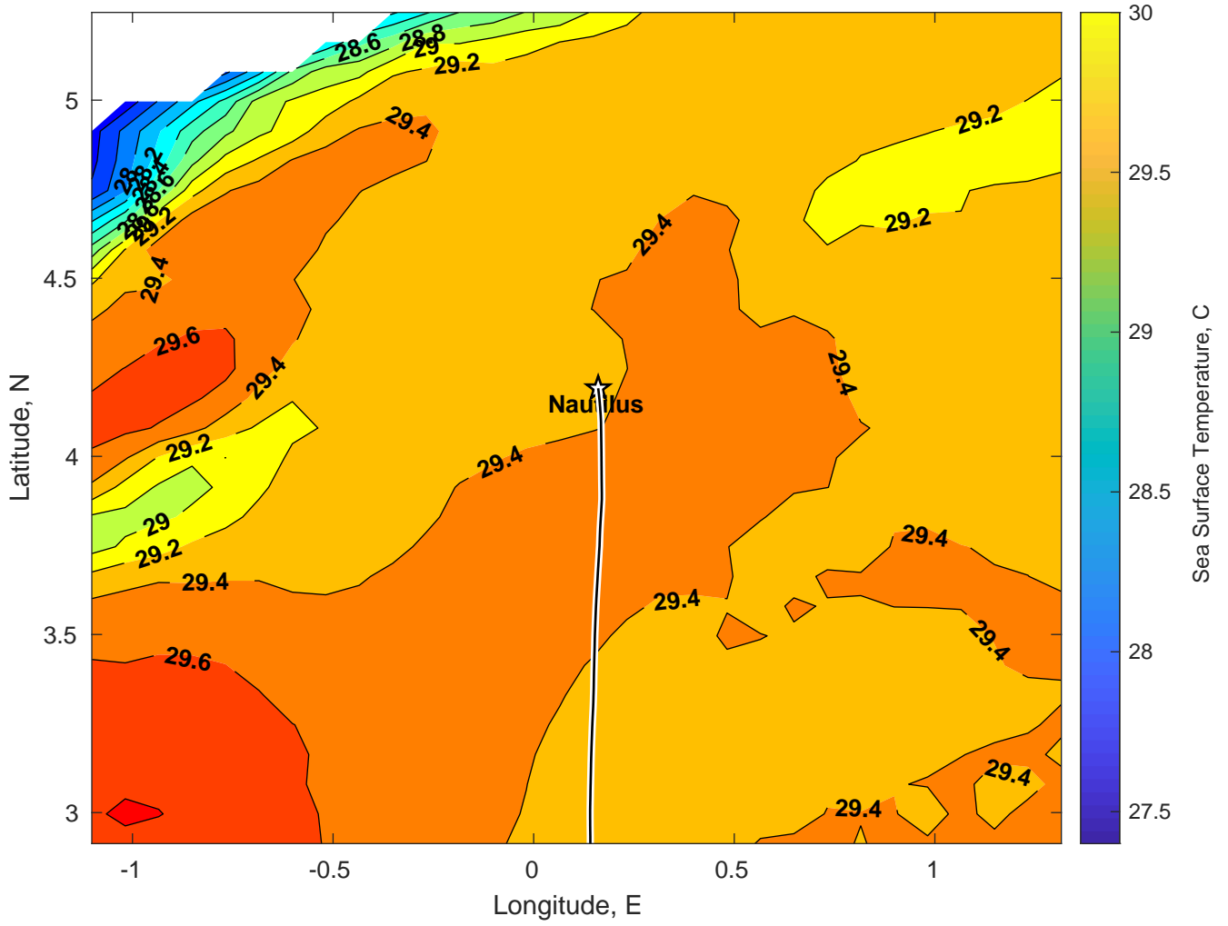
SST for Nautilus at 23-Mar-2025 00:00:00
