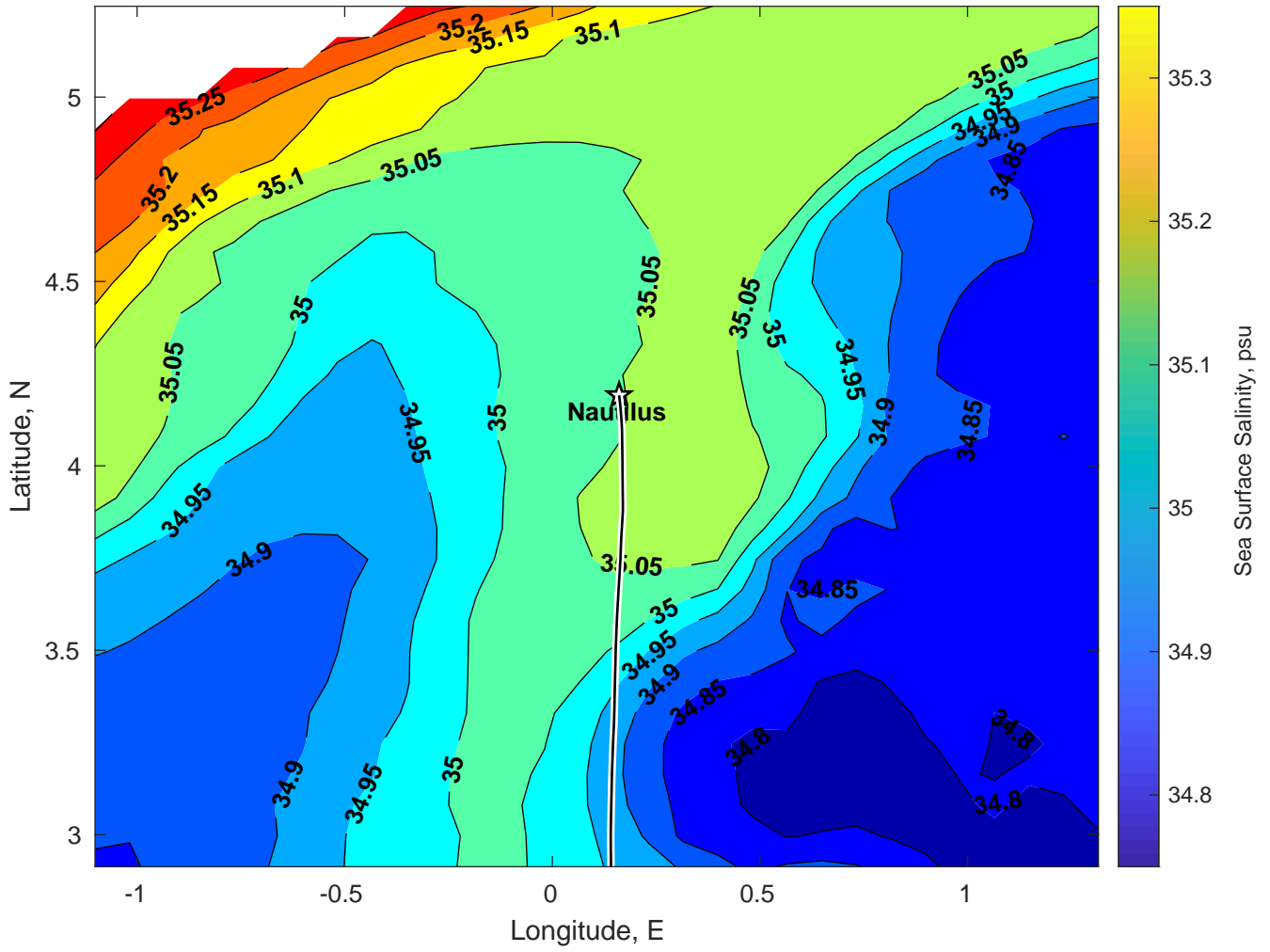
Surface Salinity for Nautilus at 23-Mar-2025 00:00:00
