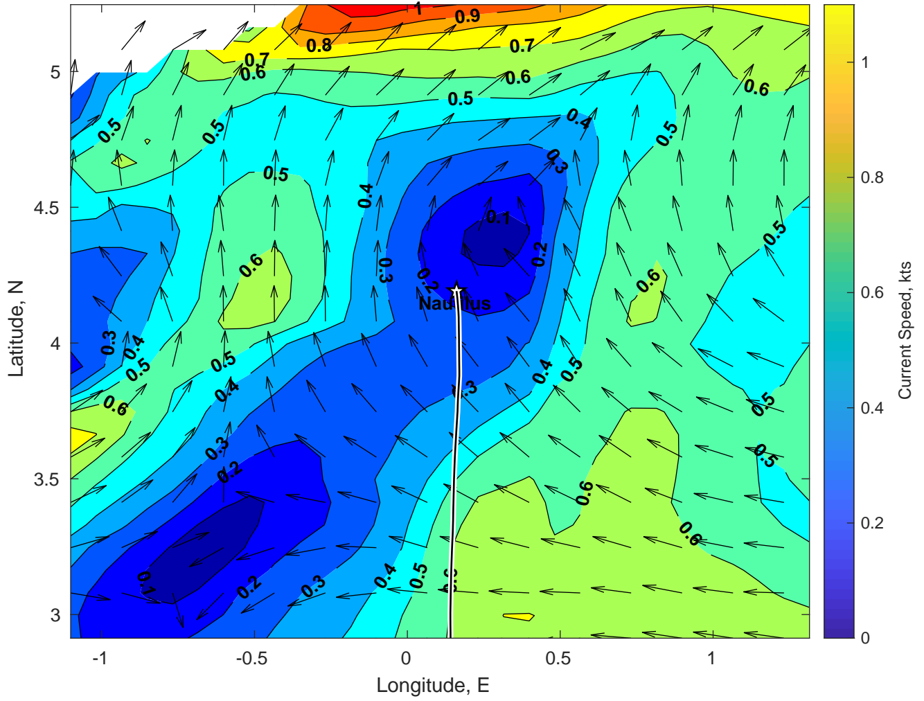
Surface Currents for Nautilus at 23-Mar-2025 00:00:00
