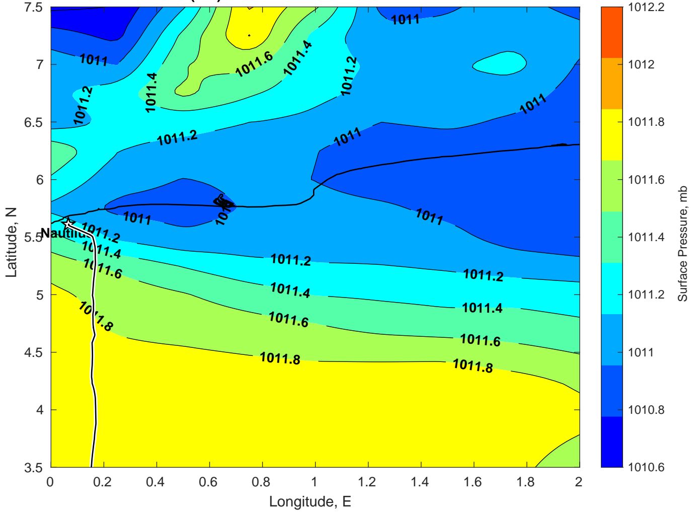
Surface Pressure (mb) for Nautilus at 24-Mar-2025 00:00:00
