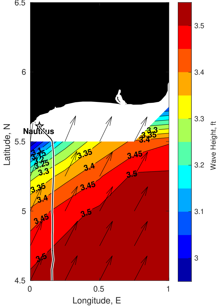
Wave Height (ft) for Nautilus at 24-Mar-2025 09:00:00
