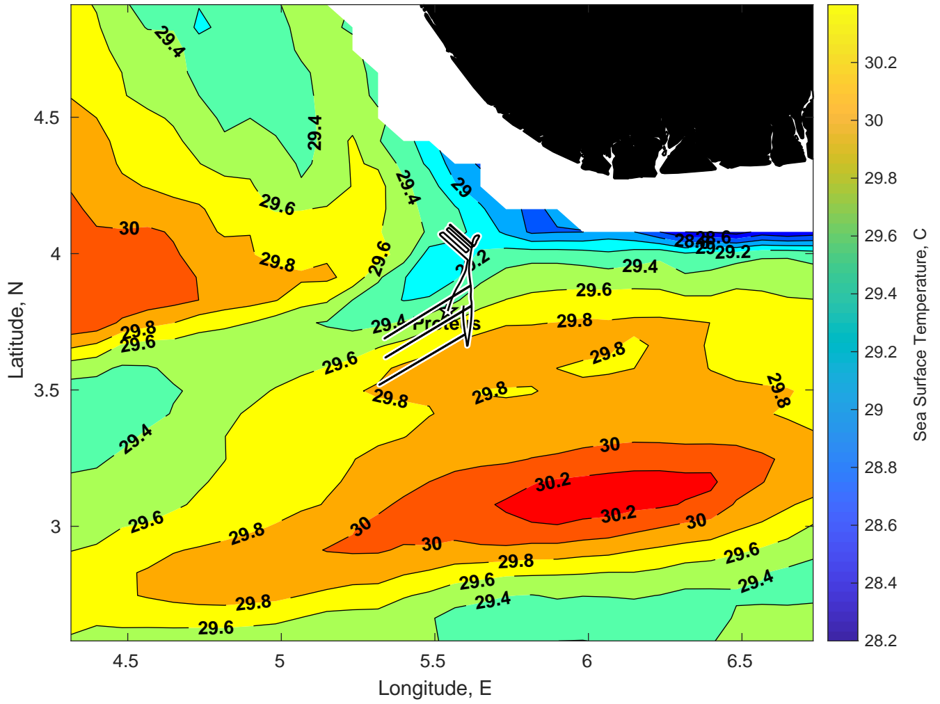
SST for Proteus at 23-Mar-2025 00:00:00
