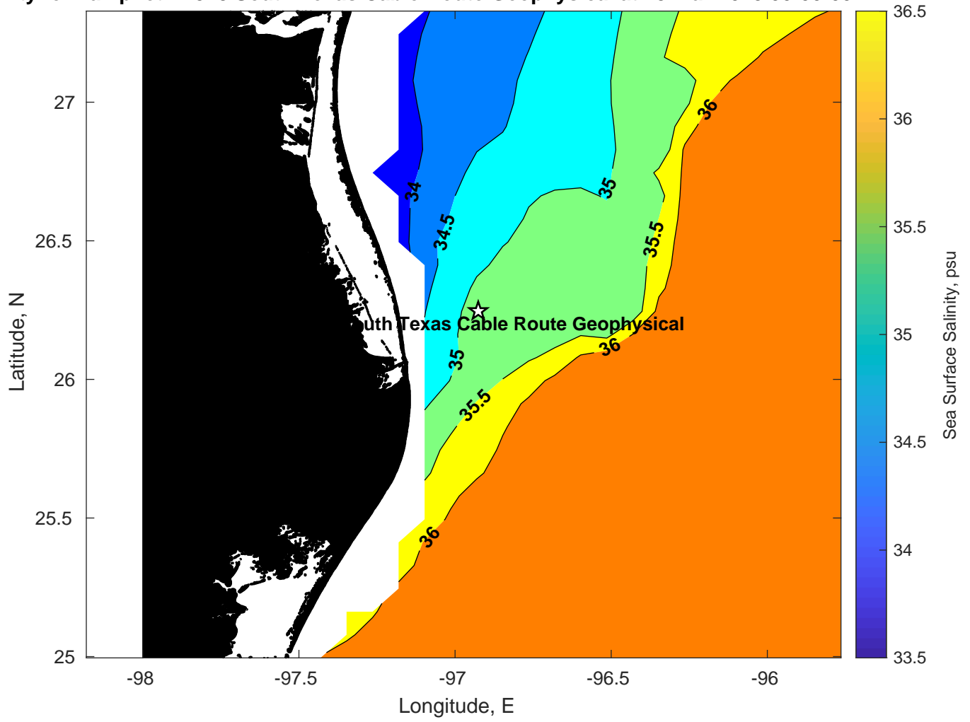
Surface Salinity for Tampnet P2378 South Texas Cable Route Geophysical at 23-Mar-2025 00:00:00
