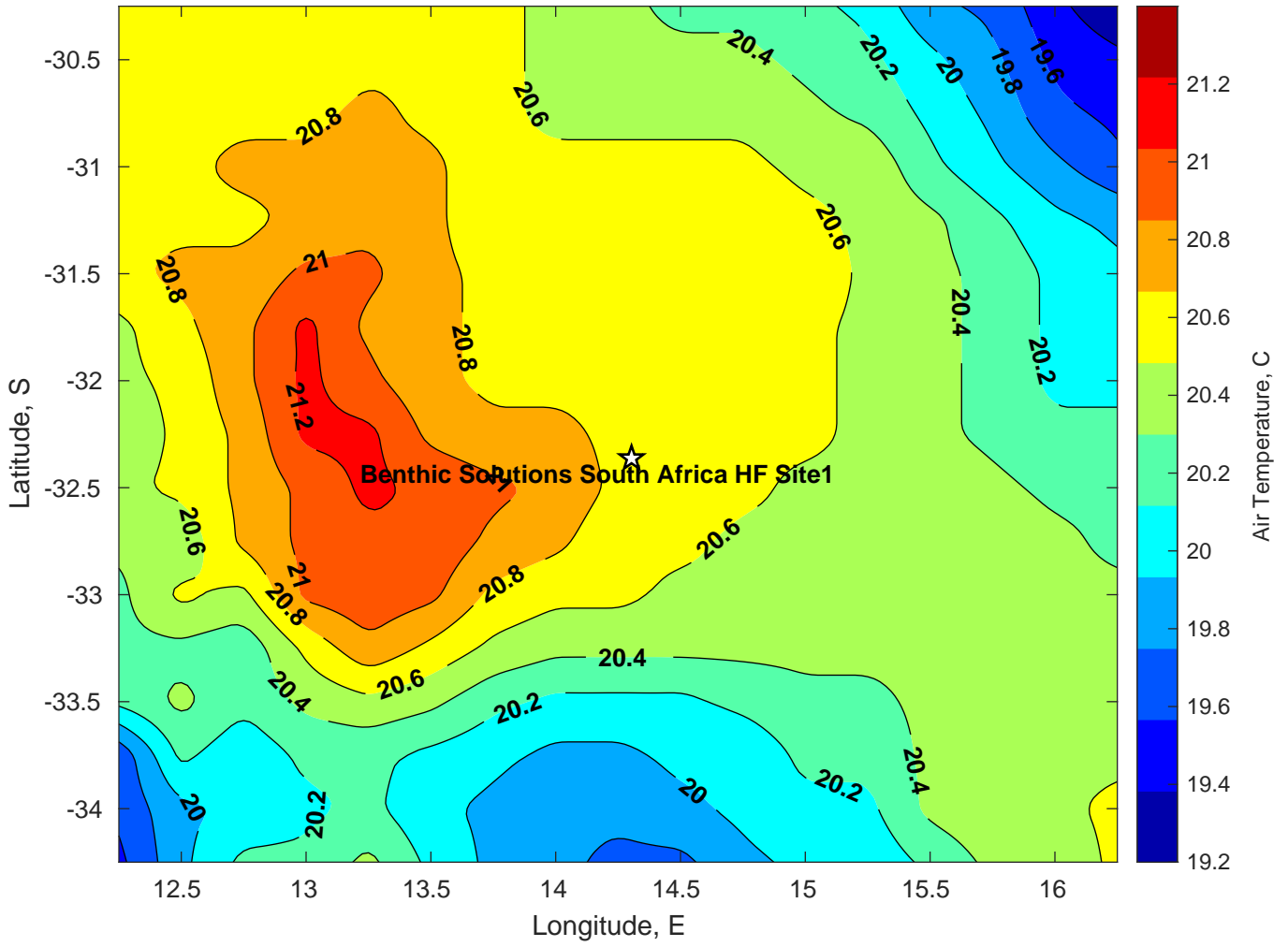
Air Temperature (C) for Benthic Solutions South Africa HF Site1 at 25-Mar-2025
