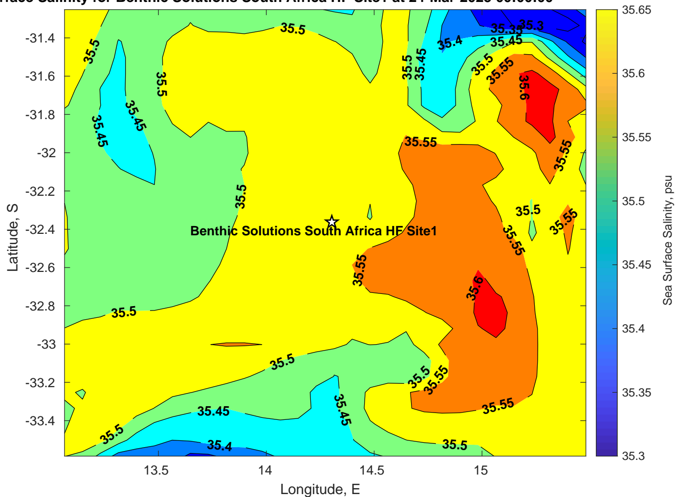
Surface Salinity for Benthic Solutions South Africa HF Site1 at 24-Mar-2025 00:00:00
