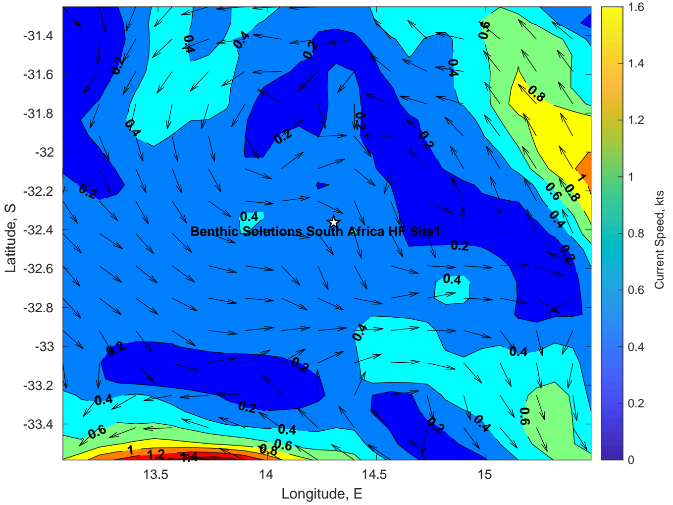
Surface Currents for Benthic Solutions South Africa HF Site1 at 24-Mar-2025 00:00:00
