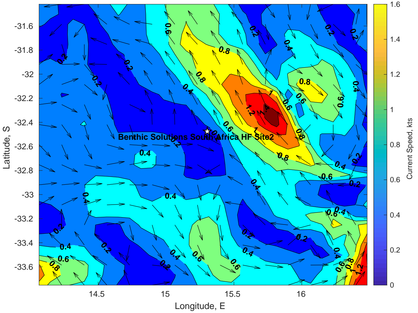
Surface Currents for Benthic Solutions South Africa HF Site2 at 24-Mar-2025 00:00:00
