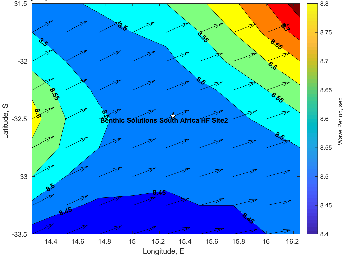
Wave Period (sec) for Benthic Solutions South Africa HF Site2 at 25-Mar-2025 09:00:00
