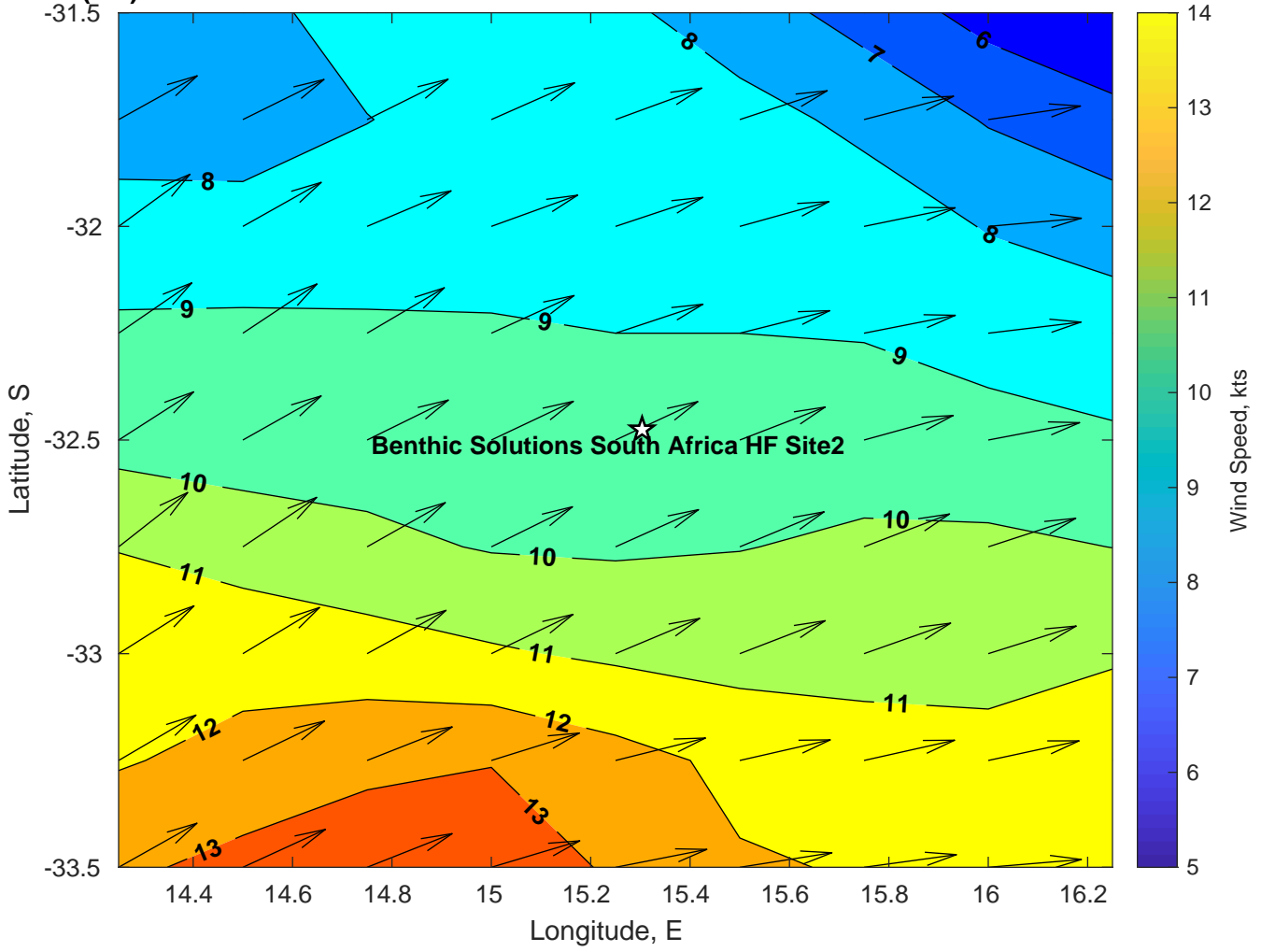
Winds (kts) for Benthic Solutions South Africa HF Site2 at 25-Mar-2025 09:00:00
